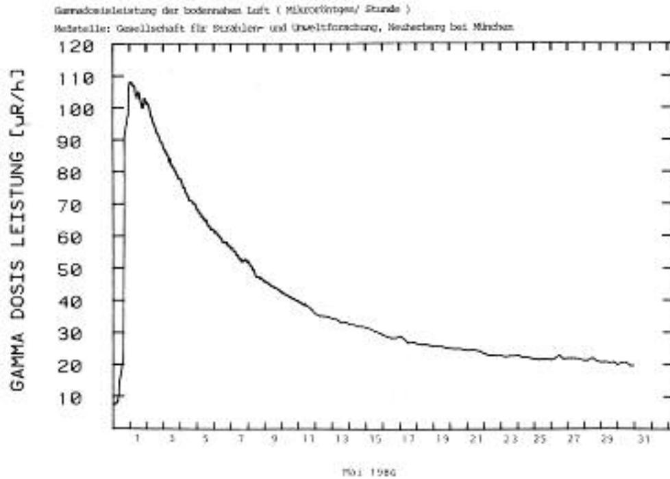
Figure 15: Gamma dose rate in the air during May 1986 in Munich, Germany. In the first days of May it reached about 110 \mu\text{R}/\text{h} , more than 10-times the normal level of 8 \mu\text{R}/\text{h} .
