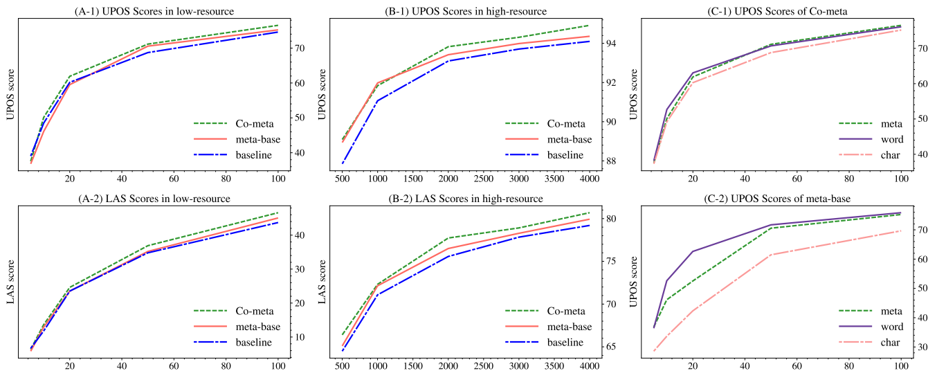
Figure 3: Evaluation results for Chinese (zh_gsd) based on the different sizes of the train set and proposed models. We apply ENSEMBLE based Co-meta with the fixed size of 12k unlabeled sentences while varying training set size.
