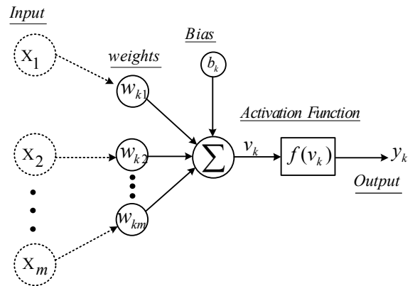
Fig. 2 Neuron model
