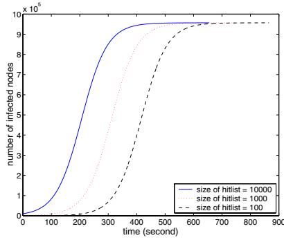
(a) Effect of Hitlist Size (All cases are without patching and take a period of one second to complete infection.)
