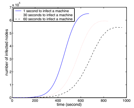
(c) Effect of Time to Complete Infection (All cases have a hitlist of 100 entries and a patching rate of 0.0005 /second.)
