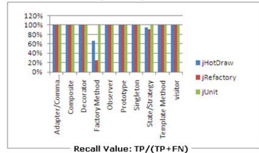
Fig 2: Results extracted from jHotDraw, jReactory, jUnit
