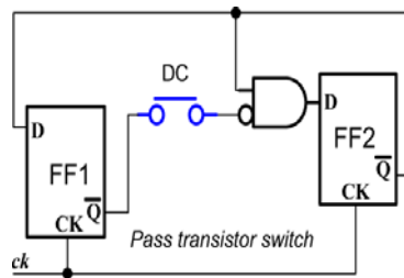
Fig.3. Logic structure of proposed 2/3 counter design
