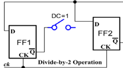
Fig.4. Divide-by-2 operation
