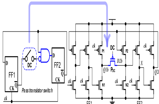
Fig.6. Schematic of proposed E-TSPC-based divide-by-2/3 counter
