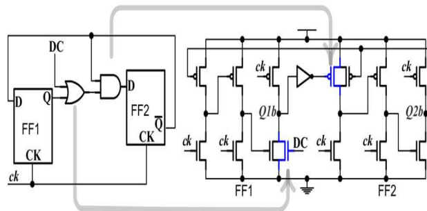
Fig.1. Previous E-TSPC-based divide-by-2/3 counter designs –design
