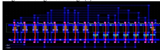
Fig.7.6(b) Layout Design
