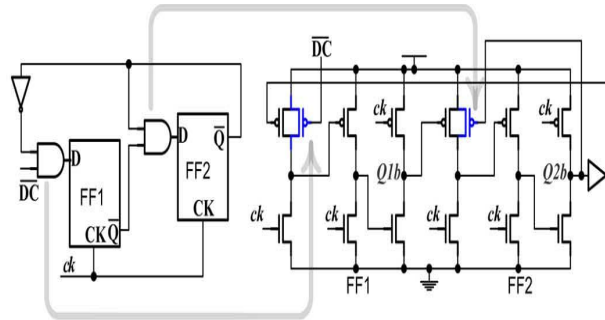
Fig.2. Previous E-TSPC-based divide-by-2/3 counter designs-design
