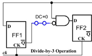
Fig.5. Divide-by-3 operation
