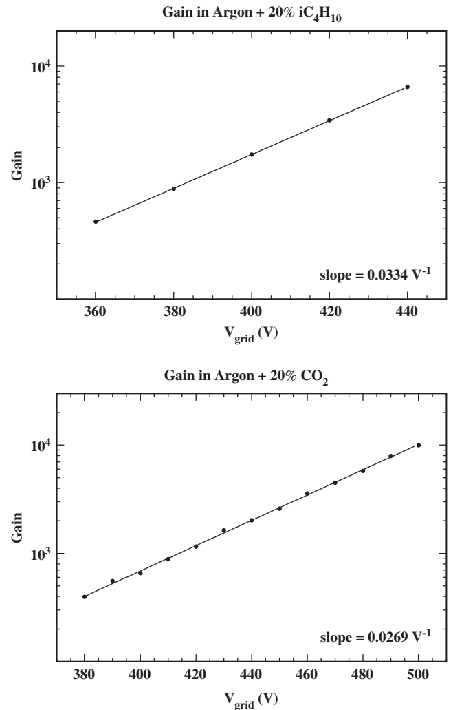
Fig. 6. Measured gas gain vs. grid voltage for Ar/isobutane 80/20 (top) and for Ar/CO 2 80/20 (bottom).
