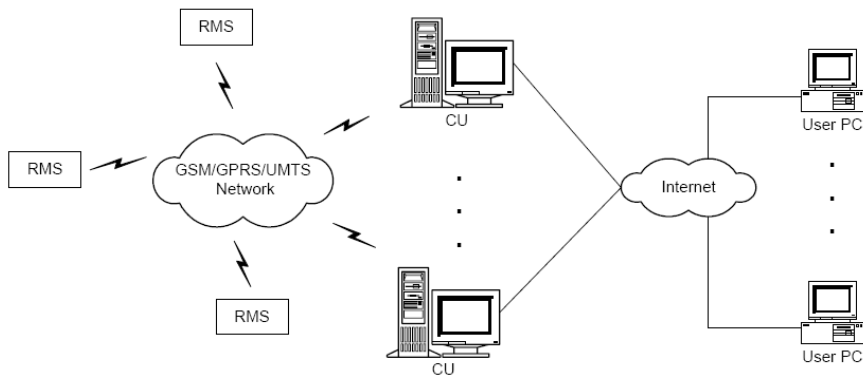
Fig. 9 – System architecture.
