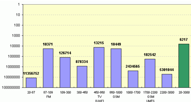
Fig. 15 – Power Density measurement results conducted with a spectrum analyzer (narrowband). The bold indicates how many times below the limit the measured levels are.
