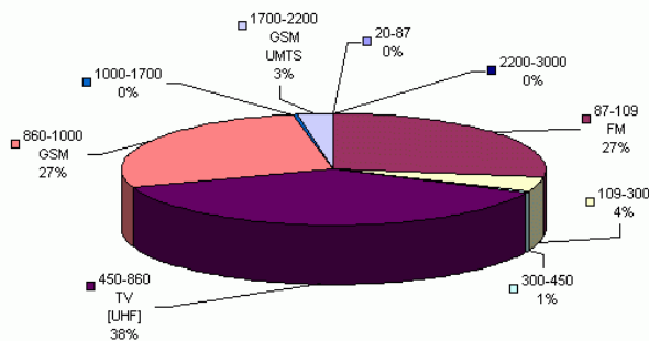
Fig. 16 – Contribution of each band to the total electromagnetic radiation calculated by spectrum analyzer measurements.
