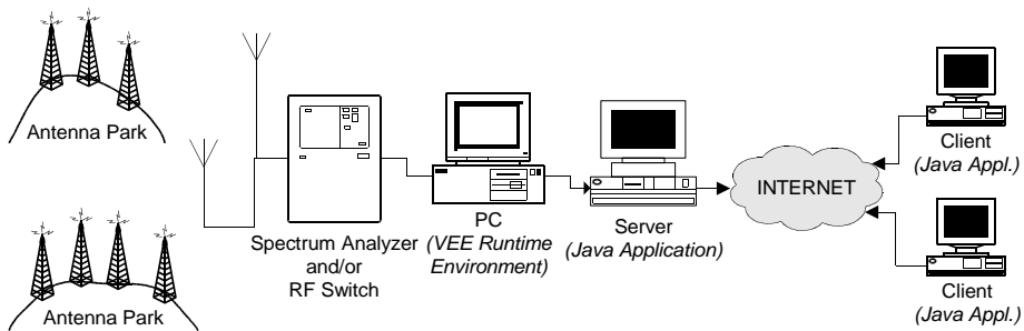
Fig. 1 – General configuration of the web-based radio monitoring system.
