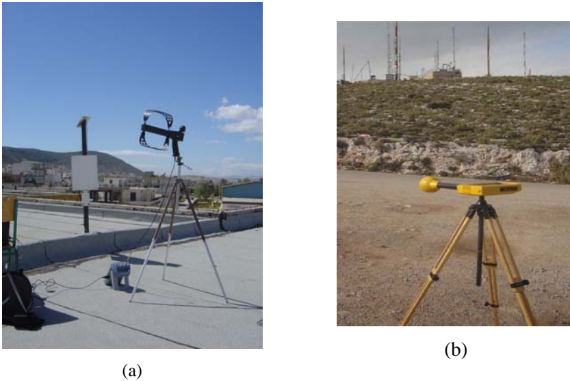
Fig. 14 – Narrowband measurement setup: (a) Spectrum analyzer ; (b) Selective radiation meter .
