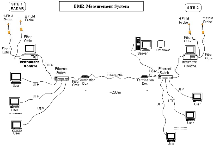
Fig. 8 – System architecture.
