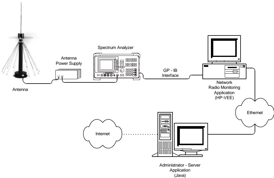
Fig. 2 – Measurement set – up.
