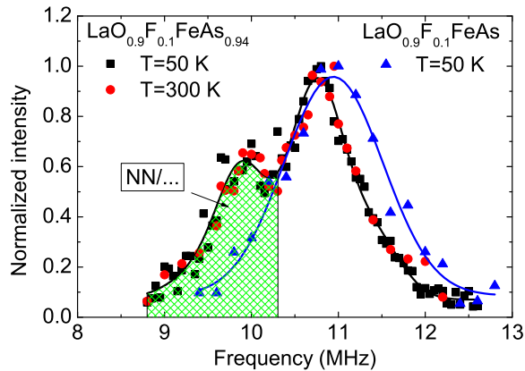
FIG. 1: (Color online) ^{75}\text{As} NQR spectrum at T = 50 K, together with the spectrum of a reference sample 17 , and room-temperature measurements 18 . Black line: a typical fit according to an As-vacancy arrangement shown in Fig. 2. Blue line: broad single-peak fit of the NQR-spectrum of a reference sample. NN/... and the shaded green area indicate schematically the low-frequency spectral weight below about 10.3 MHz suggested for the NN and NNN shells around an AV as shown in Fig. 2.
