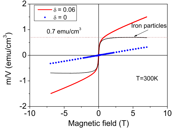
FIG. 4: (color online) Field dependence of the magnetization of \text{LaO}_{0.9}\text{F}_{0.1}\text{FeAs}_{1-\delta} at 300 K.
