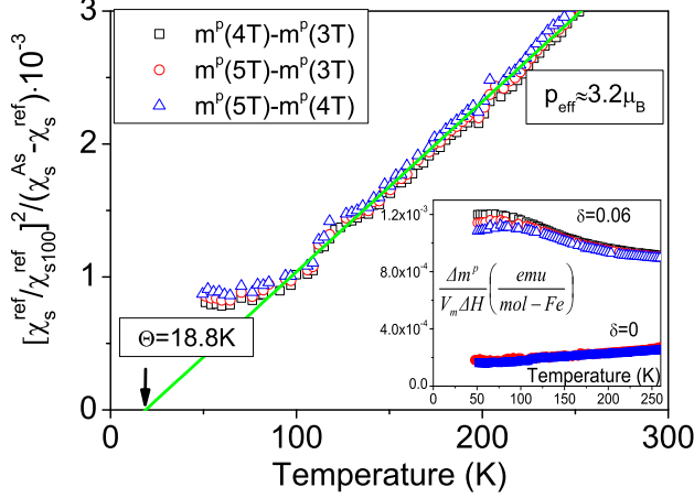
FIG. 6: (Color online) The T -dependence of the ratio \left[\frac{\chi_s^{\text{ref}}(T)}{\chi_s^{\text{ref}}(T_{\text{ref}})}\right]^2 \cdot \frac{1}{\chi_s^{\text{As}}(T) - \chi_s^{\text{ref}}(T)} for \text{LaO}_{0.9}\text{F}_{0.1}\text{FeAs}_{1-\delta} , where \chi_s^{\text{ref}} and \chi_s^{\text{As}} are spin susceptibilities of the \text{LaO}_{0.9}\text{F}_{0.1}\text{FeAs} and \text{LaO}_{0.9}\text{F}_{0.1}\text{FeAs}_{0.94} . Straight line is a fit by Eq. (3.6). Details of the fitting procedure are described in the text. The ratio \frac{\Delta m^p}{V_m \Delta H} \left(\frac{\text{emu}}{\text{mol-Fe}}\right) for two samples defined by Eq. (3.2) is shown in the inset. The closed symbols correspond to \text{LaO}_{0.9}\text{F}_{0.1}\text{FeAs} data for the m^p(4\text{T}) - m^p(3\text{T}) and m^p(2\text{T}) - m^p(1\text{T}) .
