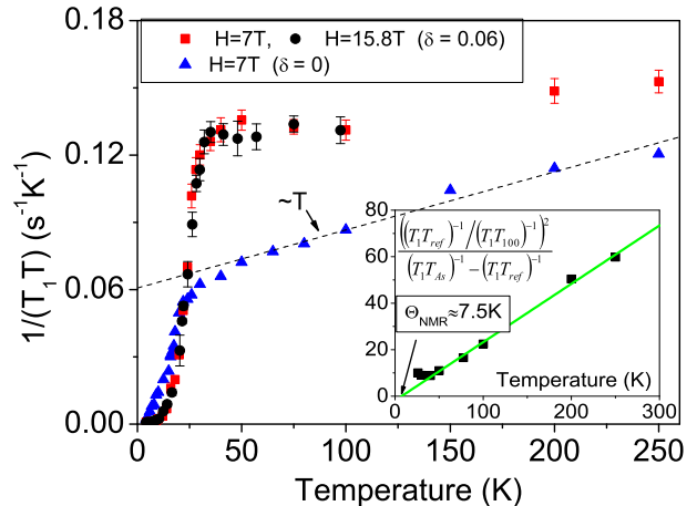
FIG. 8: (Color online) ^{75}\text{As} spin-lattice relaxation rate 1/T_1T versus temperature in \text{LaO}_{0.9}\text{F}_{0.1}\text{FeAs}_{1-\delta} . The data are taken from Ref. 12. The step decrease of both curves reflects the onset of the superconducting transition. The inset shows the T -dependence of the ratio \frac{((T_1T_{\text{ref}})^{-1}/(T_1T_{100})^{-1})^2}{(T_1T_{\text{As}})^{-1} - (T_1T_{\text{ref}})^{-1}} with (T_1T_{\text{ref}})^{-1} , (T_1T_{100})^{-1} as the nuclear spin-lattice relaxation rates of \text{LaO}_{0.9}\text{F}_{0.1}\text{FeAs} at arbitrary temperature and at T_{\text{ref}} = 100 K, respectively, and with (T_1T_{\text{As}})^{-1} as the relaxation rate of \text{LaO}_{0.9}\text{F}_{0.1}\text{FeAs}_{0.94} . Details of the fitting procedure are described in the text.
