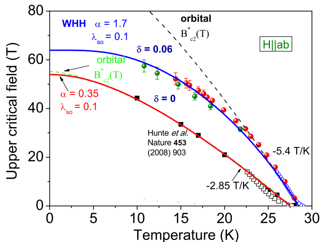
FIG. 9: (color online) Temperature dependence of the upper critical field of \text{LaO}_{0.9}\text{F}_{0.1}\text{FeAs}_{1-\delta} . Open circles: DC data, closed circles: pulsed field measurements. Green and red closed circles stand for two different samples from the same batch with the same As-deficiency measured at the FZ Dresden and the IFW Dresden, respectively 35,36 . For comparison, the upper critical field data reported in Ref. 13 are shown (closed squares). Open squares: DC data of the reference sample measured at the IFW Dresden 36 . Solid lines: fit of the experimental data to the WHH model. Dashed lines: the orbital upper critical field B_{c2}^*(T) .
