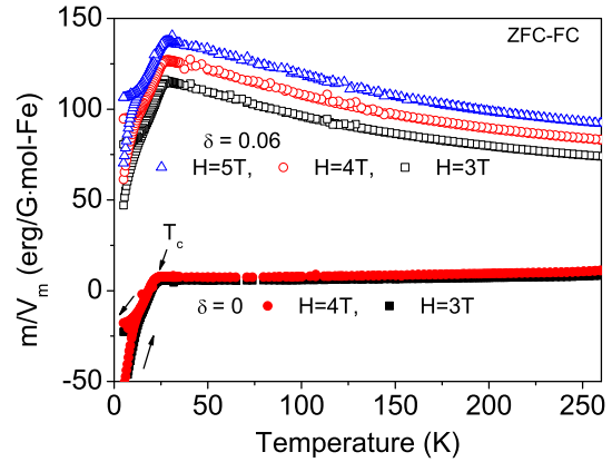
FIG. 3: (color online) Temperature dependence of the magnetization after zero-field cooling at different magnetic fields for \text{LaO}_{0.9}\text{F}_{0.1}\text{FeAs}_{1-\delta} .
