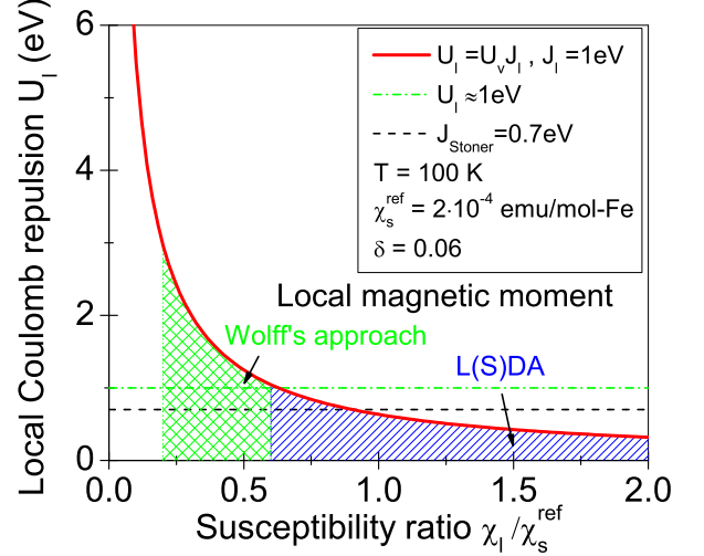
FIG. 7: (Color online) The local Coulomb repulsion for a localized state created by an As vacancy according to Eq. (3.8). The green line denotes the critical strength of U_l where the formation of a local moment at iron sites surrounding an As-vacancy sets in according with the Wolff's model. Noteworthy, we admit that local moments can exist also below U_l = 1 \text{eV} . According to L(S)DA calculations reported in Ref. 31 the formation of the local moments can be expected also in a weakly correlated situation since there is no correlation in the L(S)DA approach.
