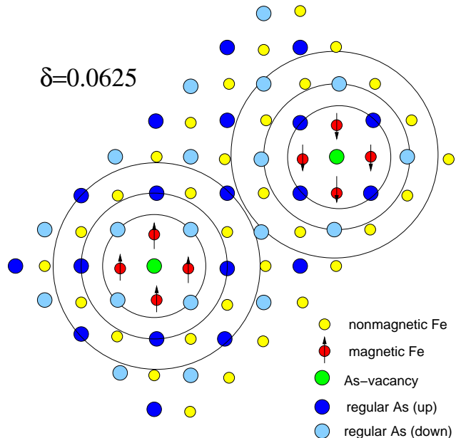
FIG. 2: (Color online) Schematic structure of an FeAs-block with two neighboring As vacancies (AV) at a concentration of \delta = 0.0625 , i.e. in the range suggested by the NQR-data shown in Fig. 1 for a typical As-deficient sample. The low-frequency spectral weight below 10.3 MHz is attributed to NN and NNN-shells around an As-vacancy (AV) whereas the high-frequency part is attributed to more distant As sites. Notice the four Fe-sites surrounding an AV involved in a local moment. The local magnetic moments are depicted for the simplest case where only the first neighbor shell around an AV is affected (see also text).
