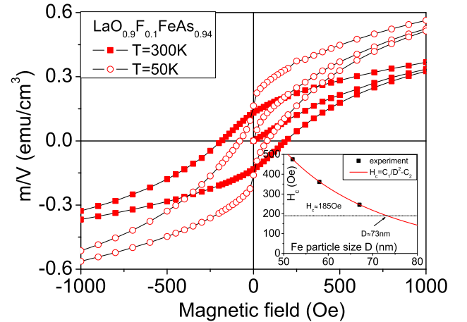
FIG. 5: (color online) Field dependence of the magnetization of \text{LaO}_{0.9}\text{F}_{0.1}\text{FeAs}_{0.94} . Inset: Coercive field H_{\text{cor}} of iron particles vs. particle size (these experimental data are taken from Ref. 21 ). The intercept between the fit curve and the horizontal line at 185 Oe gives the minimum size of the iron particles in the \text{LaO}_{0.9}\text{F}_{0.1}\text{FeAs}_{0.94} sample.
