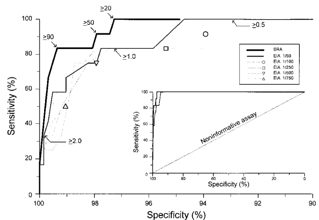
Figure 2. Comparison of activation and antigen assays for HIT by receiver operating characteristics (ROC) curve analysis. For the orthopedic patients, the activation and antigen assays are compared at various cutoff points between negative and positive results. Activation assay (SRA, serotonin release assay, thick solid line). Although the sensitivity-specificity trade-off analysis was performed at 5% increments of serotonin release, the data points for cutoff 20% or more, 50% or more, and 90% or more serotonin release are shown. Antigen assay (EIA, enzyme immunoassay, thin solid line indicating standard dilution of blood sample 1/50; thin broken lines indicating higher dilutions [1/100, 1/250, 1/500, 1/750], as indicated). Although the sensitivity-specificity trade-off analysis was performed at 0.1-OD increments, the data points for cutoff of 0.5 or more, 1.0 or more, and 2.0 or more are shown. The ROC curve analysis suggests that both the activation and the antigen assays are highly informative for diagnosing HIT in this patient population. For comparison, the inset shows the full-scale ROC curve analysis for both activation and (at conventional 1/50 dilution) antigen assays together with a (theoretical) noninformative assay (shown as dashed line). The data indicate that the operating characteristics of the antigen assay are not improved by performing the assay using a greater dilution of patient serum/plasma.
