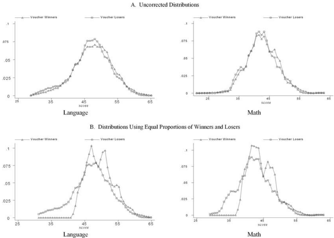
FIGURE 2. TEST-SCORE DISTRIBUTIONS
