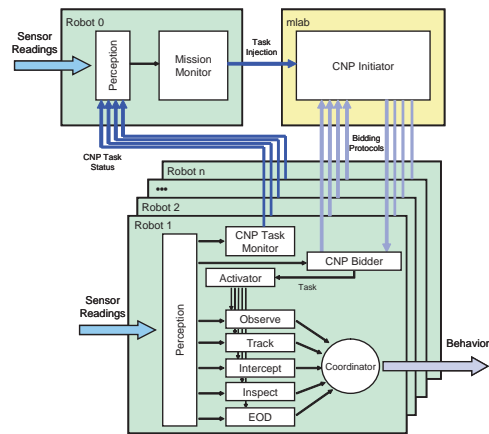
Fig. 14. Architectural framework of the execution phase for the CBR and runtime-CNP design
