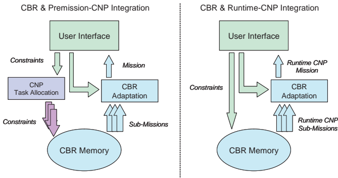
Fig. 5. Alternative integration designs: (L) CBR and permission-CNP and (R) CBR and runtime-CNP
