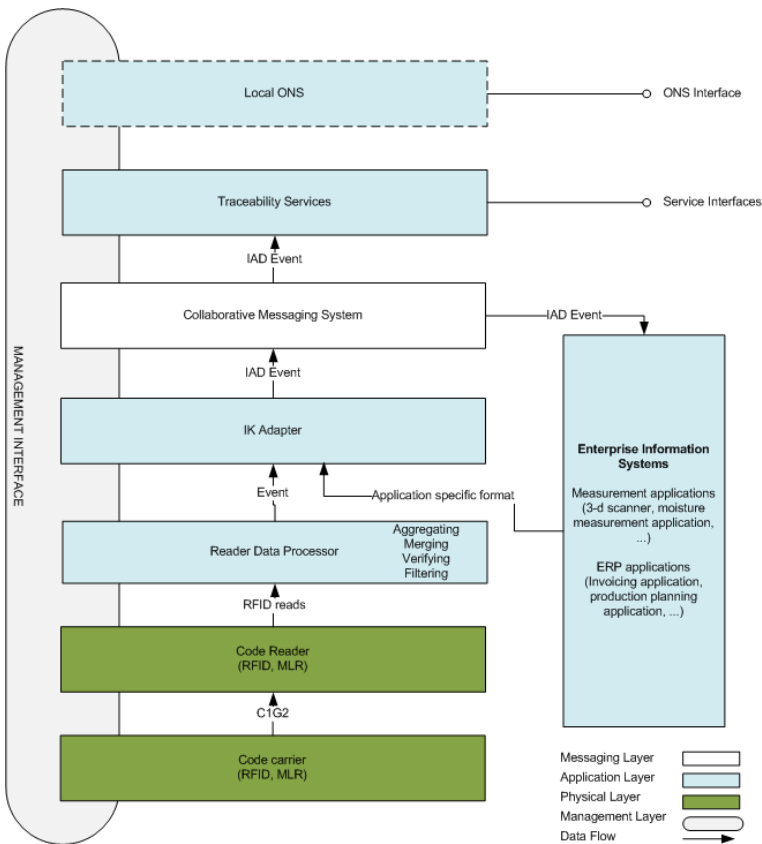
Figure 11. ICT System Architecture.
