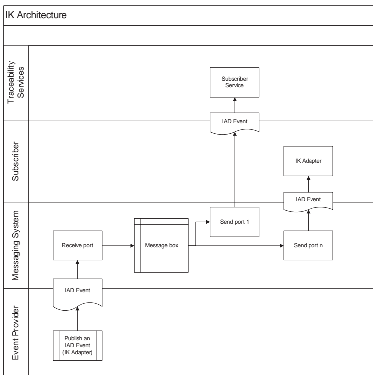
Figure 13. Collaborative Messaging System Data Flow.
