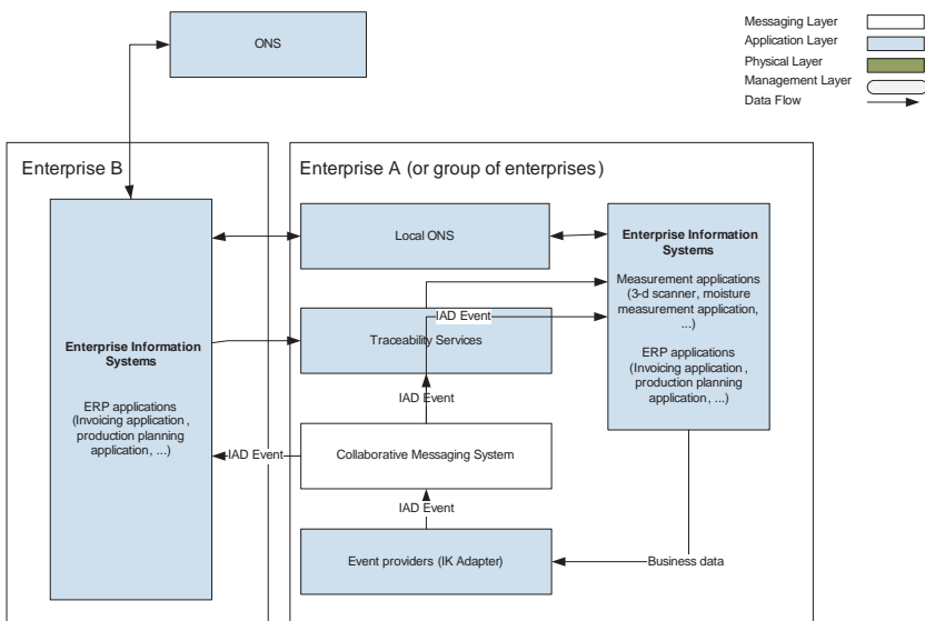
Figure 12. ICT system architecture across enterprises.
