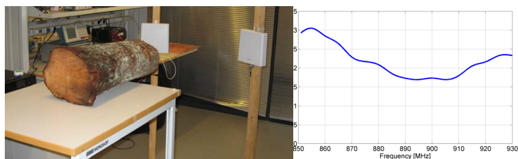
Figure 8. The reading range measurement in the laboratory and the measured reading range.
