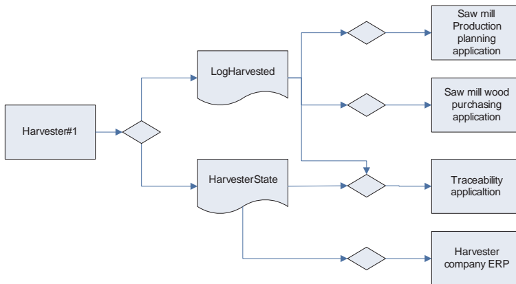
Figure 14. Example IAD event data flow.
