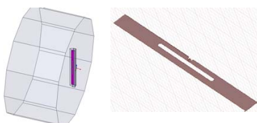
Figure 7. Simulation model of the transponder inside a log and the planar dipole antenna layout.
