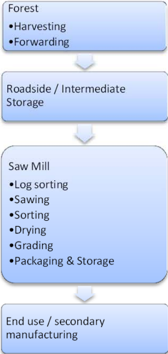
Figure 2. Nordic wood supply chain for sawn timber.
