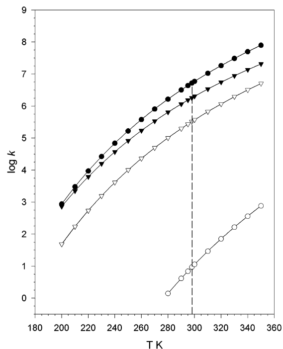
Figure 2. Thermal unimolecular rate constants for N-C_{\alpha} bond dissociations in 3a (○), 4b (●), 6a (▼), and 6d (▽).
