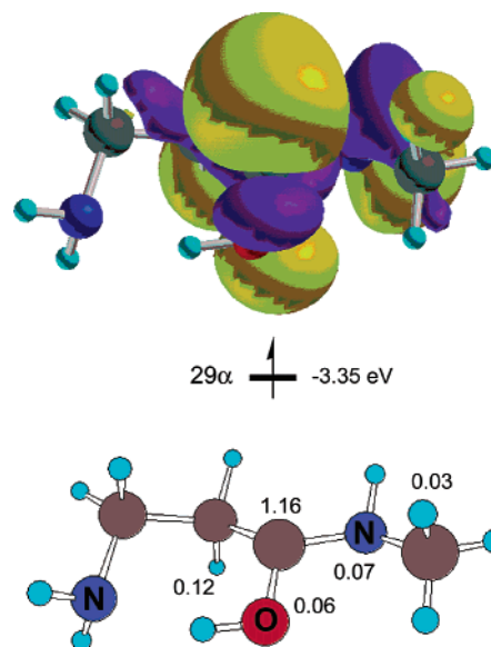
Figure 1. Atomic spin densities and singly occupied molecular orbital ( 29\alpha ) in 1a .
