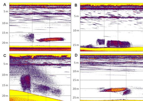
Figure 1 Responses of sprat schools to sound exposure. A: Small school, cut off abruptly after the beginning of the sound. B: Medium sized school cut off at the onset of the sound. C: Large sprat school cut off at the onset of the sound. D: Small sprat school increasing in density in response to sound exposure. A vertical line indicates the beginning and end of each sound sequence.
