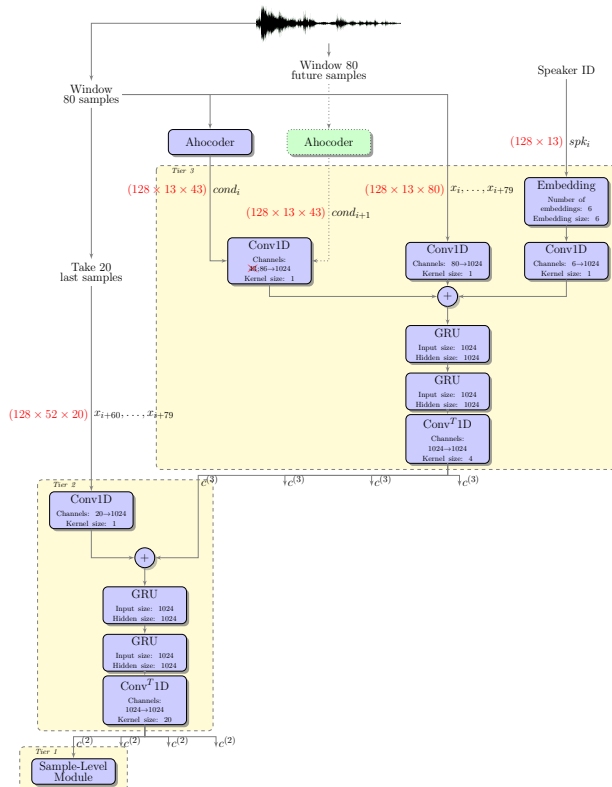
Figure 3: Conditioned SampleRNN with multi-speaker adaptation
