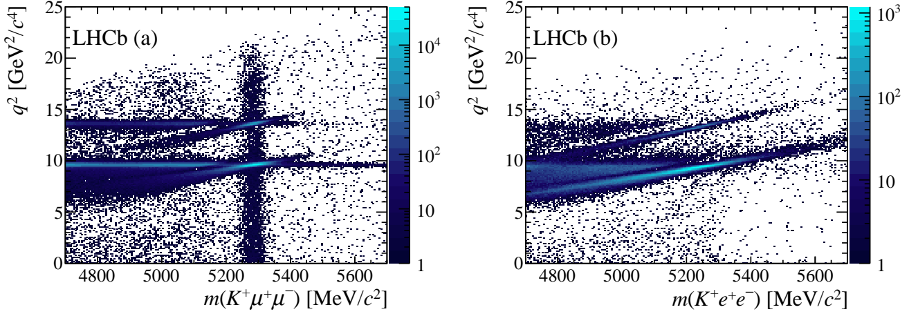
Figure 1: Dilepton invariant mass squared, q^2 , as a function of the K^+\ell^+\ell^- invariant mass, m(K^+\ell^+\ell^-) , for selected (a) B^+ \rightarrow K^+\mu^+\mu^- and (b) B^+ \rightarrow K^+e^+e^- candidates. The radiative tail of the J/\psi and \psi(2S) mesons is most pronounced in the electron mode due to the larger bremsstrahlung and because the energy resolution of the ECAL is lower compared to the momentum resolution of the tracking system.
