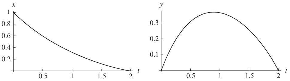
Figure 5. The graphs of x = f_x(t) (left) and y = f_y(t) (right)
