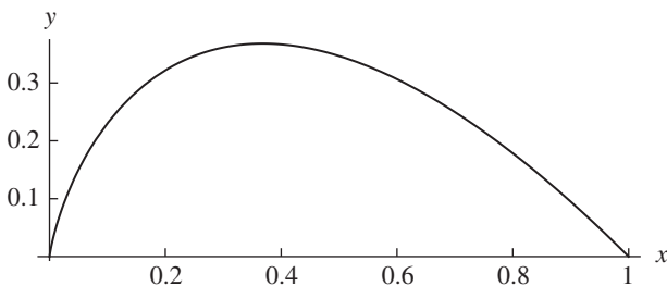
Figure 4. The graph of y = -x \ln x
