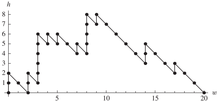
Figure 2. A pill-bottle walk with n = 20
