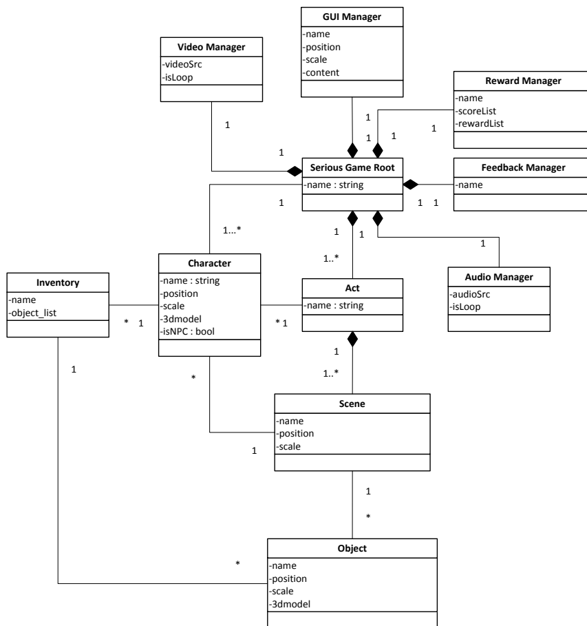
Figure 2: Meta model of GLiSMo's structure modeling
