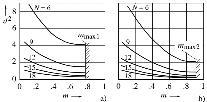
Fig. 19: Synchronized carrier modulation, loss factor d^2 versus modulation index; (a) suboscillation method, (b) space vector modulation
