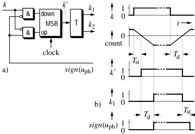
Fig. 33: Dead-time compensation; (a) compensation and delay circuit per phase, (b) signal waveforms; T: interlock circuit
