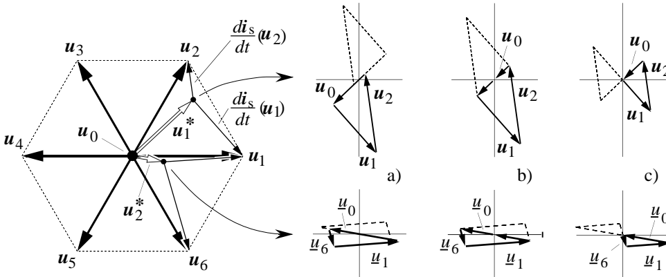
Fig. 15: Linearized trajectories of the harmonic current for two voltage references u_1^* and u_2^* : and (a) suboscillation method, (b) space vector modulation, (c) modified space vector modulation
