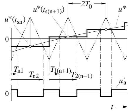
Fig. 16: Synchronized regular sampling
