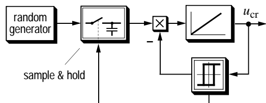
Fig. 20: Random frequency carrier signal generator
