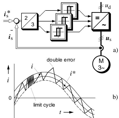
Fig. 34: Hysteresis current control; (a) signal flow diagram, (b) basic current waveform-
