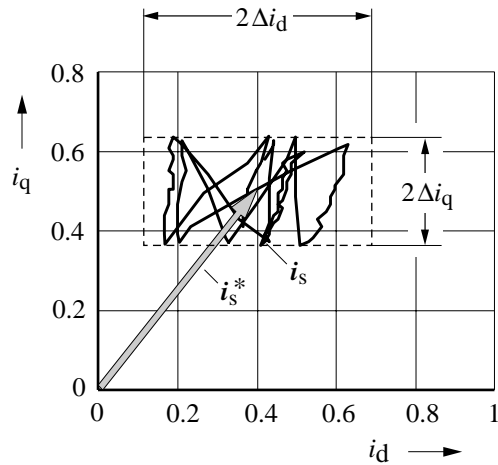
Fig. 44: Pulseshape modulation with field orientation
