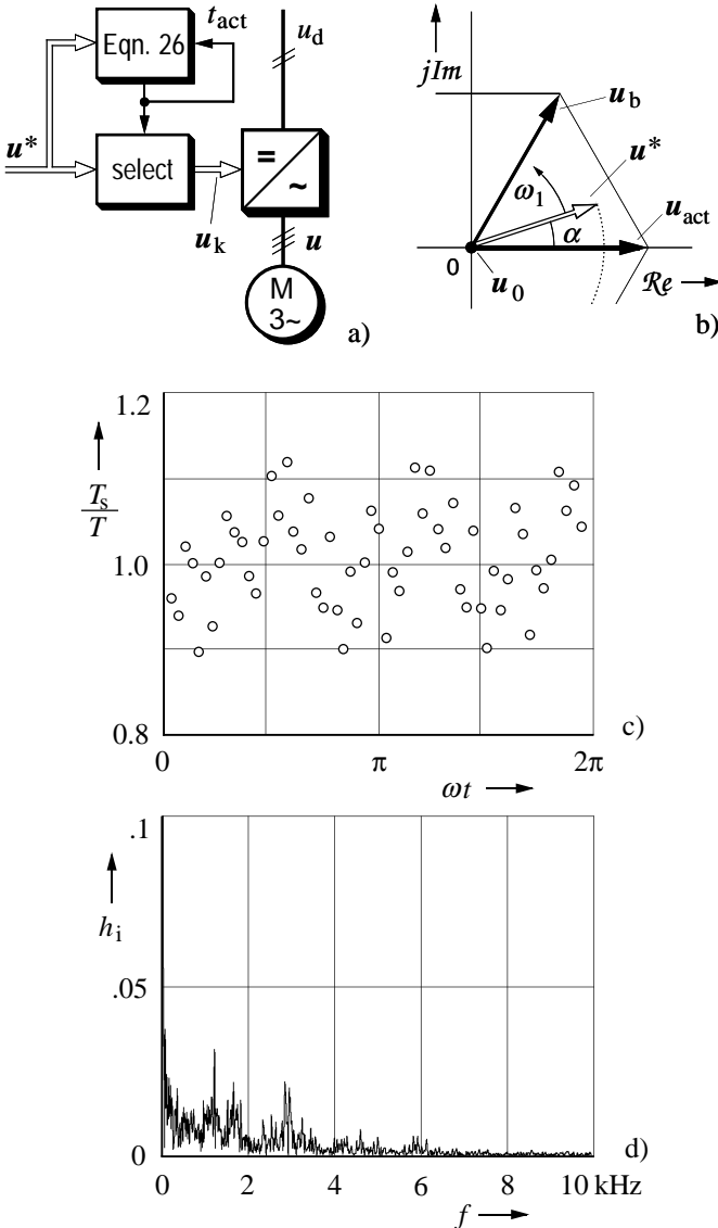
Fig. 21: Carrierless pulsewidth modulation; (a) signal flow diagram, (b) switching state vectors of the first 60^\circ -sector, (c) measured subcycle durations, (d) harmonic spectrum
