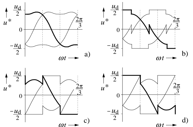
Fig. 10: Reference waveforms with added zero-sequence systems; (a) with added third harmonic, (b), (c), (d) with added rectangular signals of triple fundamental frequency
