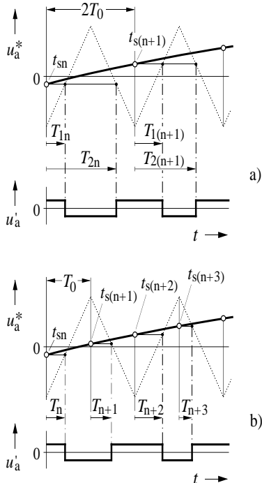
Fig. 12: Sampling techniques; (a) symmetrical regular sampling, (b) asymmetric regular sampling
