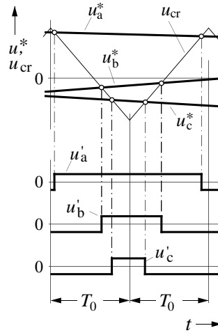
Fig. 9: Determination of the subcycle duration. Note that the three phase potentials u_a^* , u_b^* , u_c^* are of equal magnitude at the beginning and
