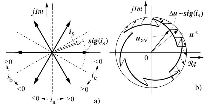
Fig. 30: Dead-time effect; (a) location of the polarity vector \mathbf{sig}(\mathbf{i}) , (b) trajectory of the distorted average voltage \mathbf{u}_{av}
