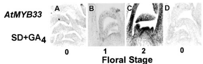
Figure 8. Increase in expression at the shoot apex of AtMYB33 with GA_4 induced flowering of plants in SDs. Sixty-day-old plants were treated twice over 4 d with GA_4 (66 ng plant -1 ). Expression of AtMYB33 is shown at the start of treatment (A), at 8 d (B), or 12 d (C) and in D for a sense probe of an apex harvested 8 d after the start of treatment. Floral scores are based on the scale proposed by Smyth et al. (1990).
