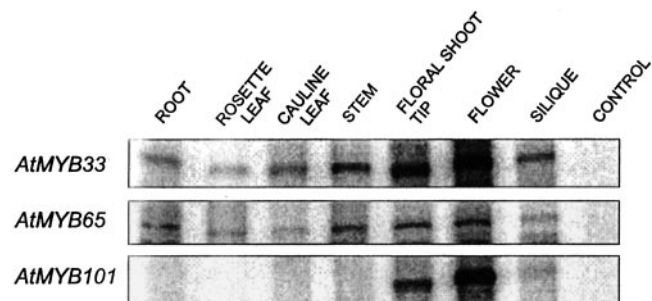
Figure 3. Expression pattern of Arabidopsis GAMYB-like genes, AtMYB33 , AtMYB65 , and AtMYB101 , as determined by RNase protection assays of mRNA levels in various tissues from Columbia plants. The negative control for the RNase protection assay contained only yeast tRNA. The floral shoot tip included flower clusters at the tip of the inflorescence but with no visible petals.
