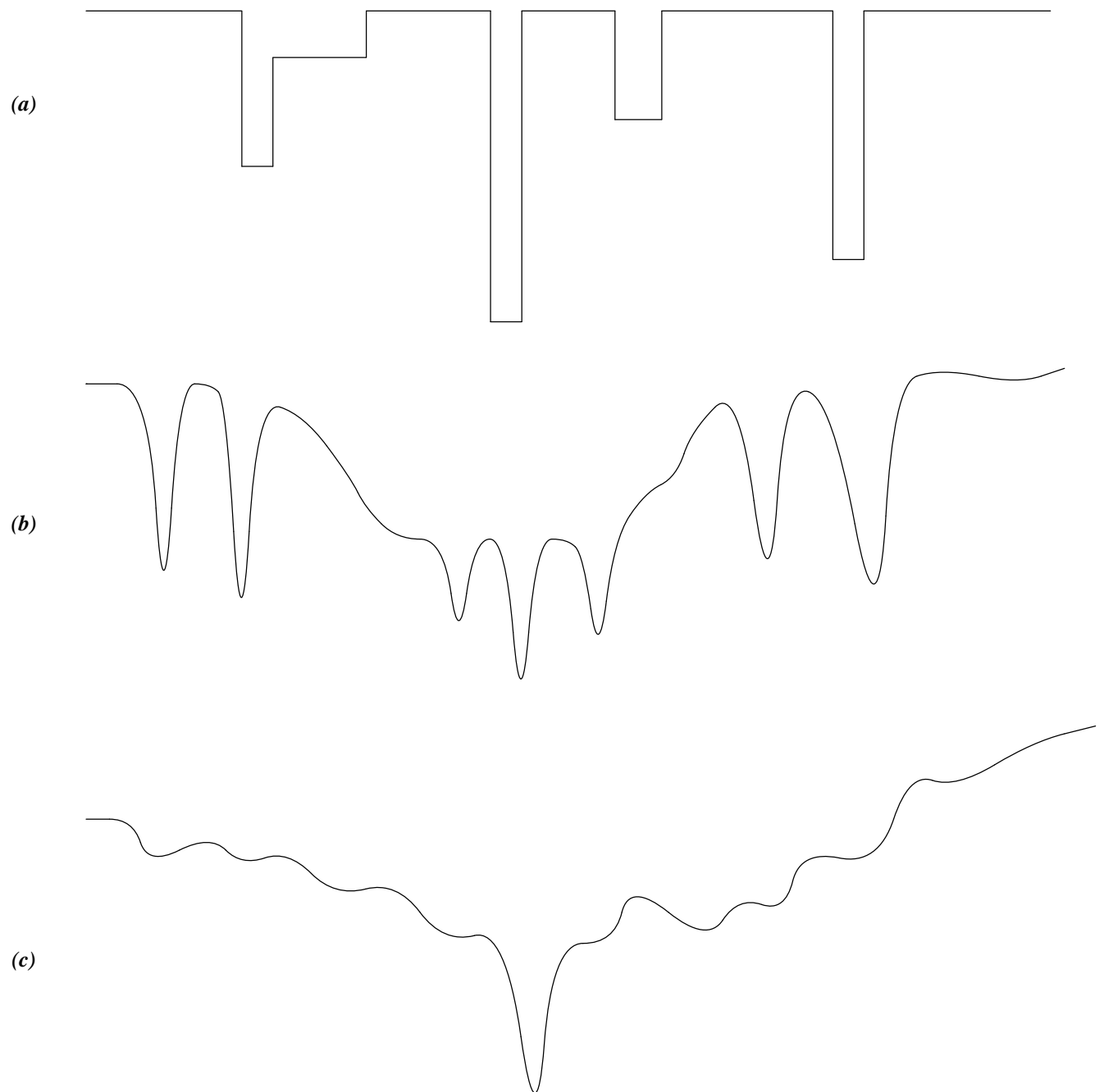
FIGURE 2: Examples of objective function variation for simulated annealing; (a) A "golf course" surface with no features except for objective function minima, (b) objective function with deep basins of attraction about suboptimal minima, (c) Objective function with shallow basins about suboptimal minima and a deep basin about the optimum.
