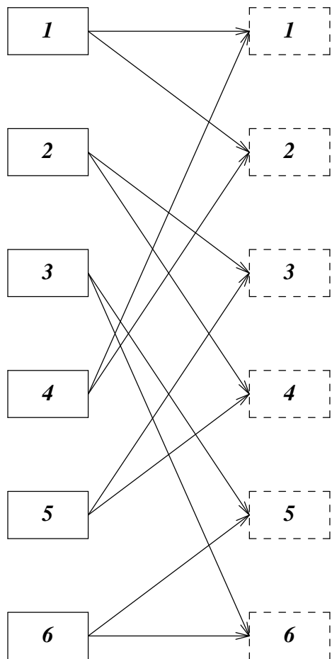
FIGURE 3: The perfect shuffle network with N=6 nodes and L=Np=12 links.
