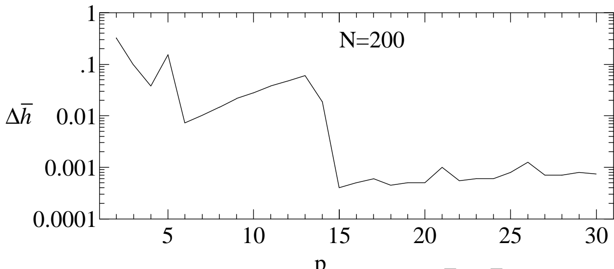
FIGURE 7: A plot of the difference in \bar{h} ( \Delta \bar{h} ) between the perfect shuffle network and the Moore bound versus p .
