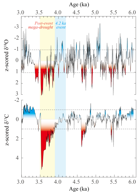
Figure 3. Inferred hydro-climatic variability at Rodrigues from 6 to 3 ka. LAVI-4 \delta^{18}\text{O} and \delta^{13}\text{C} record are z-score transformed. Inferred droughts ( z\text{-score} > 1 ) and pluvial episodes ( z\text{-score} < -1 ) are shaded (increasing saturation index indicates increasing intensity). Dashed lines indicate 1 standard deviation. The blue bar marks the classical 4.2 ka event interval and the yellow bar marks the “post-event” mega-drought, inferred from LAVI-4.
