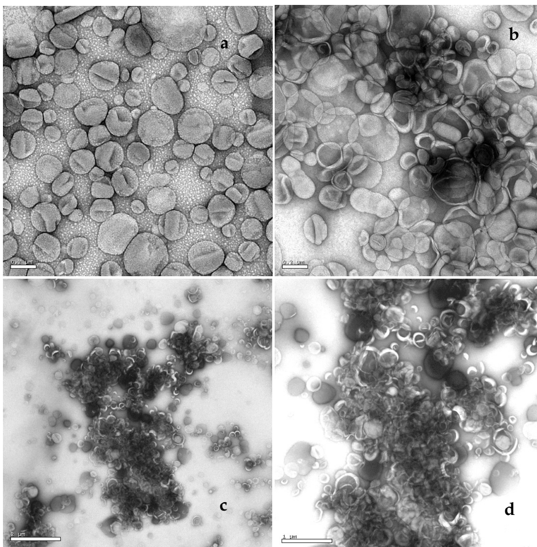
Figure 3 Negative stain electron microscope images (1% uranyl acetate) taken on a JEOL JEM 1230. (a) liposomes at 10 K magnification, scale bar 0.2 μm; (b) agglomerate at 10 K magnification, scale bar 0.2 μm; (c) agglomerate at 2 K magnification, scale bar 2 μm; (d) agglomerate at 4 K magnification, scale bar 1 μm.
