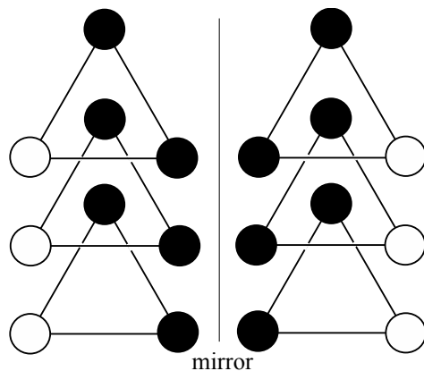
Figure 3. Overlap of Al atoms in stacked layers of kaolinite. Black circles indicate occupied Al site, and white circles indicate vacant Al sites [62].
