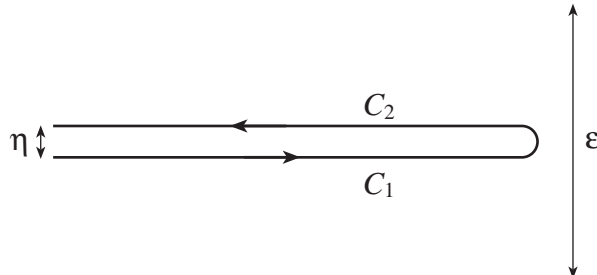
Fig. 5: The zig-zag loop; the loop goes in one direction along C_1 and comes back along C_2 . The two segments C_1 and C_2 are parallel and their distance \eta is less than the gauge theory UV cutoff \epsilon .
