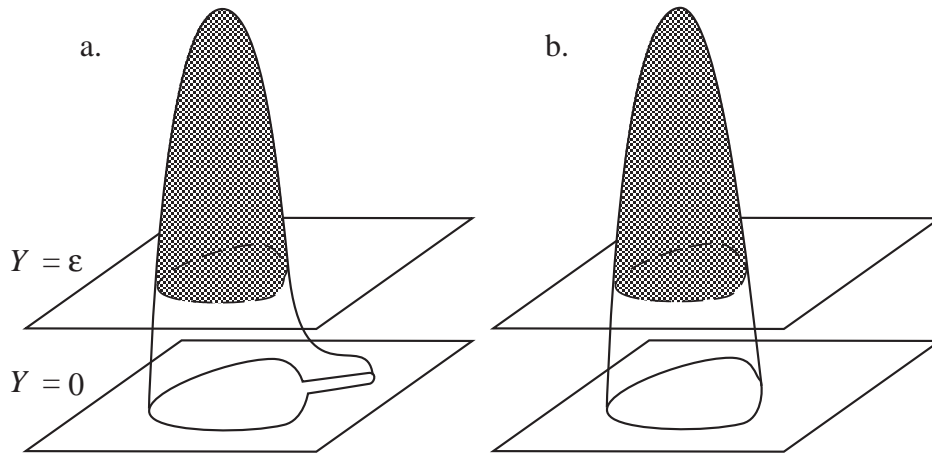
Fig. 6: The area of a loop with a zig-zag (a) is roughly the same as the loop without it (b).
