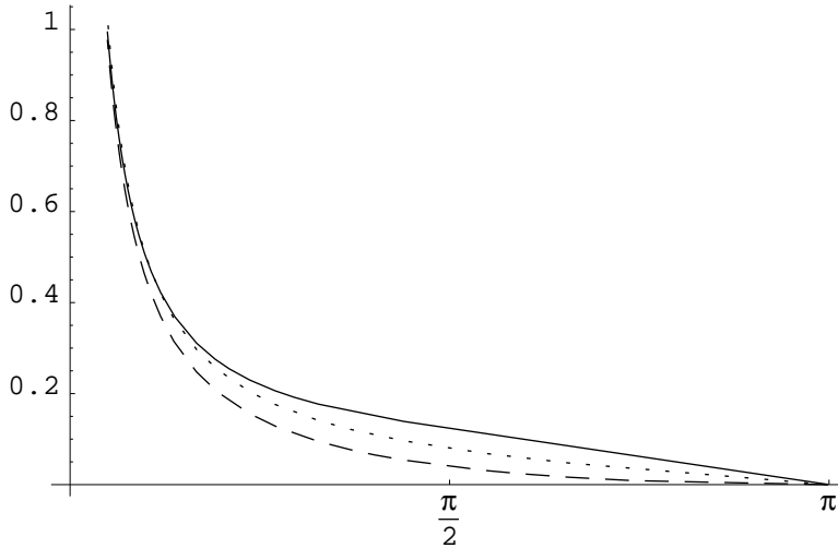
Fig. 3: The solid curve shows the function F(\Omega, 0)/2\pi , which appears in the logarithmic divergence of the minimal surface with the cusp of angle \Omega . This is compared with the perturbative result (2.12) at the cusp shown in the dashed curve. The dotted curve is half of the perturbative result (2.13) at an intersection.
