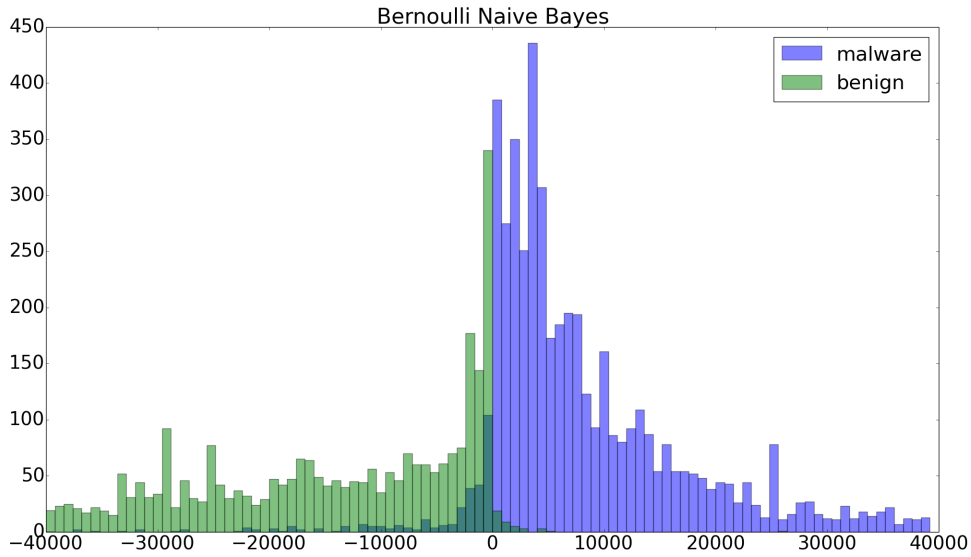
Figure 2: The histogram of log-factor sums D(f) for malicious and benign test files using Bernoulli NB. The intersection between two histograms is quite skewed. It is more difficult to find the border to get desired FNR due to the heavy-tail distribution of the intersection between two classes.
