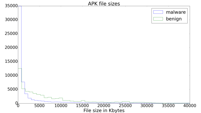
Figure 1: The histogram of APK file sizes, totally 120,000 files.
