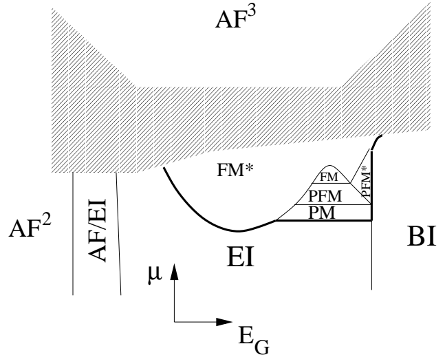
Figure 2: Partial phase diagram of the strong-coupling model as a function of E_G (half the bare splitting between a and b orbitals), and \mu , the chemical potential. The shaded region is not analyzed in this paper. Thick lines indicate the boundary between the undoped region below (with two electrons per unit cell) and the doped region above (with more than two electrons per unit cell). The AF^2 and AF^3 phases are antiferromagnetic Mott insulators with two and three electrons per unit cell, respectively. The BI state is the band insulator. Intermediate between the BI and AF^2 phases are the excitonic insulator ( EI ) and an insulator with coexisting excitonic and Néel order ( EI/AF ). The FM , FM^* , PFM , and PFM^* phases are all ferromagnetic metals (see Table 1 for the differences between these states), while PM indicates a paramagnetic metallic phase. All the metallic states above exhibit excitonic order.
