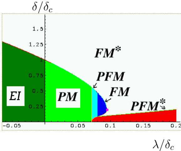
Figure 5: Free-Fermi gas approximation to the zero-temperature phase diagram. The abscissa \lambda/\delta_c is the non-dimensionalized chemical potential, and the ordinate \delta/\delta_c indicates the strength of excitonic ordering relative to super-exchange interactions (see Eqs. 29-35 for the precise definitions). The properties of the various phases shown are listed in Table 1. For larger \lambda (not shown), both excitonic ordering and ferromagnetism disappear, owing to reduction of the amplitude of \Delta .
