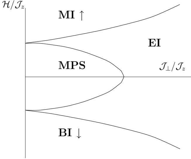
Figure 4: Mean-field phase diagram of the fully SU(4)-invariant pseudo-spin model. A large pseudo-Zeeman field (which scales linearly with the orbital splitting E_G ) stabilizes either the Mott insulating (MI) or band insulating (BI) state, depending upon its sign. For “in-plane” anisotropy ( \mathcal{J}_\perp > \mathcal{J}_z ), the intervening phase is an excitonic insulator (EI). In the opposite limit (“Ising” anisotropy) it consists of a micro-phase-separated state with a checkerboard pattern of alternating band and Mott insulating configurations at the lattice scale. In obtaining the pseudo-spin model from the strong-coupling limit of Eqs. 4-6, one finds in-plane anisotropy, and the intermediate state is expected to be excitonically ordered.
