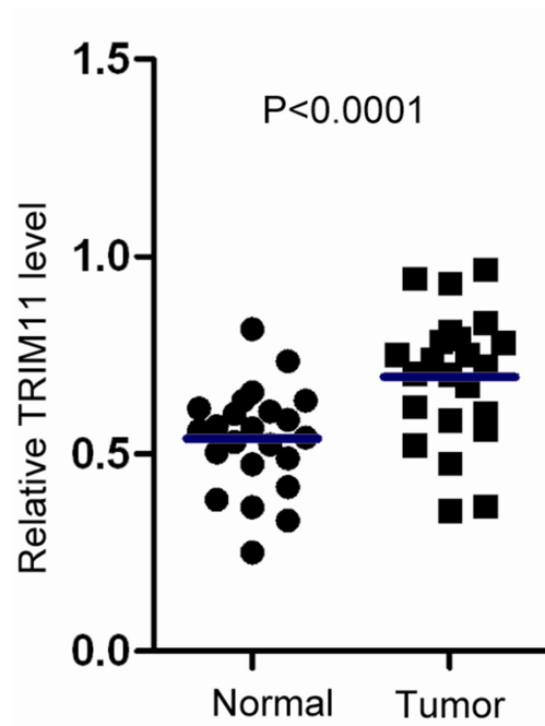
Supplementary Figure S1: Quantitative and statistical analysis of TRIM11 expression in clinical CC samples in tumor and paired normal tissues. The blue bars stand for the mean value. The p-value was calculated according to the raw data using Student's t-test ( P < 0.0001 ).
