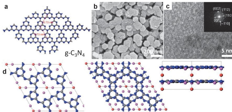
Fig. 19 Polymeric carbon nitride semiconductor from SMS. (a) Proposed structure of the ideal single layer g\text{-C}_3\text{N}_4 based on 2D arranged s -heptazine (C 6 N 7 ) units. (b) SEM and (c) TEM images of crystalline CN polymer synthesized in LiCl/KCl. (d) Proposed structure of the 2D poly(triazine imide) with intercalated Br synthesized in the salt melt of LiBr/KBr. Left: c -axis view of single layer; middle: c -axis view of two-layer stack, and right: b -axis view. Carbon, nitrogen, lithium and bromide atoms represented as grey, blue, purple and red spheres, respectively. (a–c, Reprinted with permission from ref. 158, d from ref. 160. Copyright 2008, 2013 John Wiley and Sons.)
