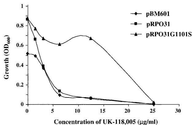
FIG. 3. Cloned mutant allele of RPO31 confers resistance to UK-118005. MIC determination for the wild-type haploid strain BY4741 containing either pBM601 (vector, no insert [◆]), p RPO31-G1101S (▲), or p RPO31 (■) after 48 h of treatment with serial dilutions of UK-118005.
