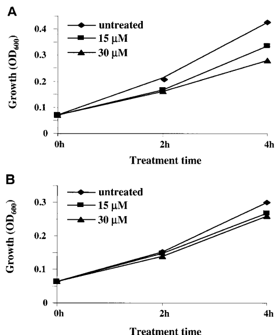
FIG. 6. Comparison of growth inhibition by UK-118005. Growth inhibition by UK-115005 in wild-type BY4741 (A) and the resistant mutant MMB2404 (B) was measured by taking OD 600 readings of the same cultures as analyzed by Northern in Fig. 5 at the times indicated. Strains were treated with 15 μM (■) or 30 μM (▲) UK-118005 or no UK-118005, i.e., the untreated control (◆).
