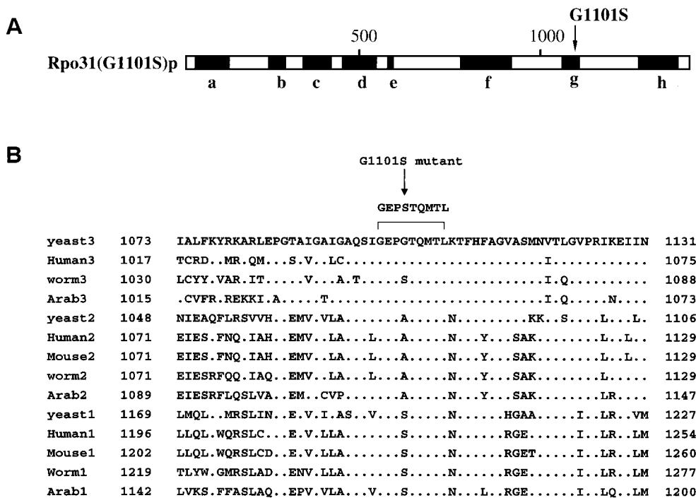
FIG. 4. (A) Site of mutation in Rpo31-G1101S mutant protein. A schematic diagram showing the eight conserved domains of Rpo31 protein and the single amino acid change from glycine (G) to serine (S) at amino acid residue 1101 in the g domain of the Rpo31 protein is shown. (B) Comparisons of homologous amino acid sequence motif g of analyzed RNA Pol large subunits from S. cerevisiae (yeast), human, mouse, Caenorhabditis elegans (worm), and Arabidopsis thaliana . The Pols from different organisms are indicated by the names of the organisms followed by 1 (Pol I), 2 (Pol II), and 3 (Pol III). Amino acid positions are given at the beginning and end of each sequence. Identical residues with the RPO31p g motif sequence (RNA Pol III) are indicated by points. The G1101S mutation site is indicated by an arrow, and its conserved surrounding amino acid residues (discussed in the text) are overlined and displayed above the overline.
