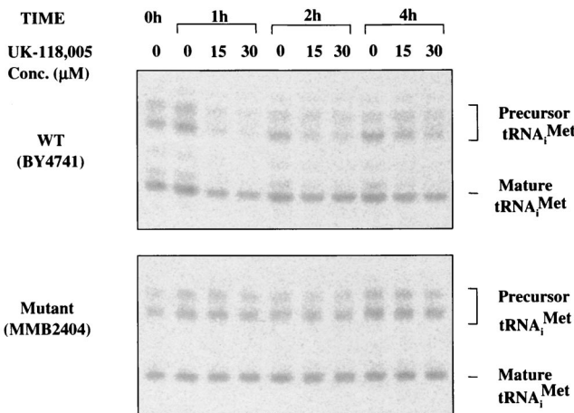
FIG. 5. Inhibition of tRNA transcription in vivo by UK-118005. A Northern blot shows a time course of treatment of wild-type BY4741 cells (top panel) and rpo31 mutant MMB2404 cells (bottom panel) either untreated (lanes 0) or treated with 15 μM or 30 μM UK-118005 as indicated (see Materials and Methods for details). The migration of the precursor and mature tRNA i Met is indicated.
