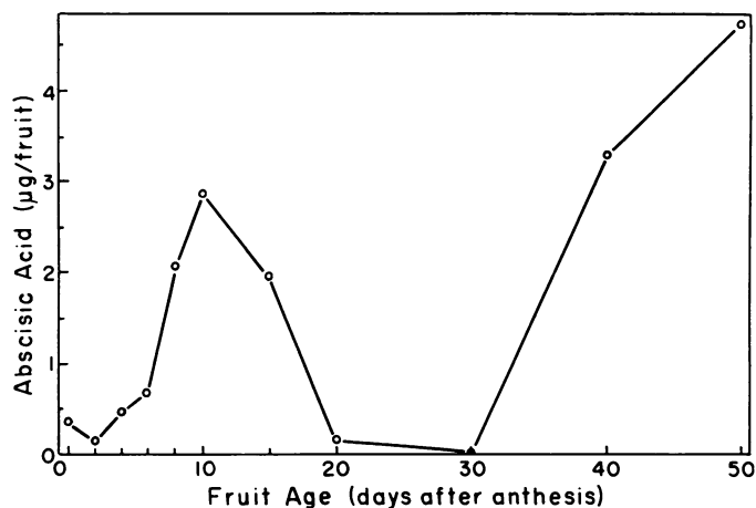
FIG. 1. Abscisic acid in cotton fruit during the course of development. Fruit were from cv. Acala SJ-1 that had flowered early in the season. Each point is the average of four determinations. Note the rapidly rising levels of ABA during the period of young fruit abscission (5th to 10th days), and during the approach of fruit wall senescence and dehiscence (30th to 50th days).
