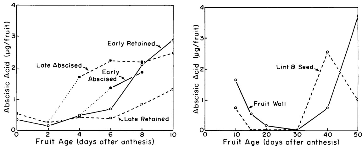
FIG. 4. Abscisic acid in "abscised" and "retained" (nonabscising) young cotton fruit of cv. Acala SJ-1, early and later in the fruiting season. Each point is the average of three or more determinations. The finely dotted lines indicate that abscission of the "early abscised" fruit did not begin until sometime between the 4th and 6th days, and abscission of the "late abscised" fruit did not begin until sometime between the 2nd and 4th days. Note the much higher levels of ABA in the late abscised fruit than in the late retained fruit. Curves for the early fruits are discussed in the text.
