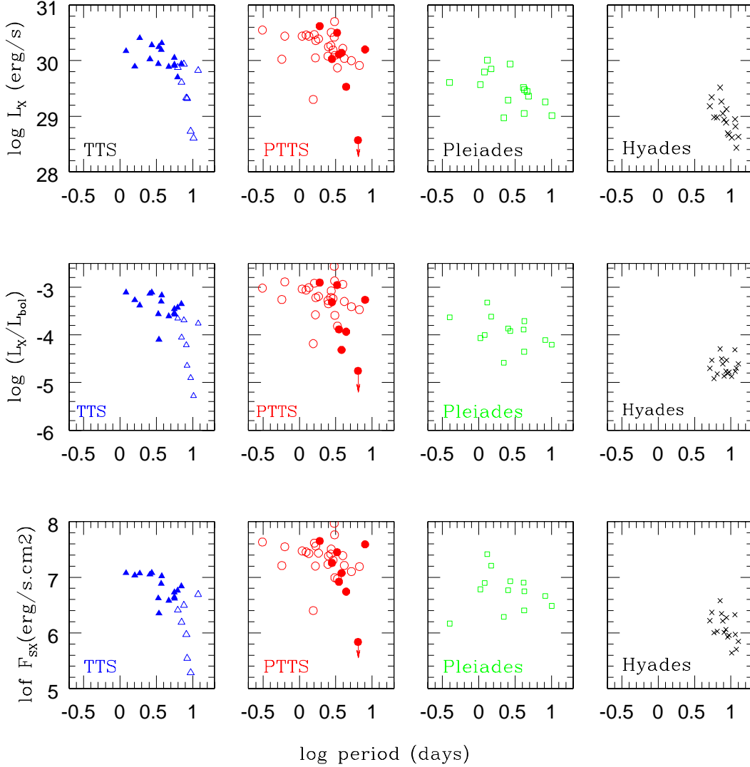
Fig. 4. Activity-rotation relations for late-type PMS and ZAMS stars with masses between 0.9\text{-}1.2M_{\odot} . We have represented TTSs in Taurus (CTTSs: open triangles, WTTSs: filled triangles), PTTSs (Lindroos: filled circles, Lupus & Taurus: open circles), Pleiades and Hyades stars. We have plotted three different activity indicators versus the rotation period: (i) X-ray luminosity (ii) X-ray to bolometric luminosity ratio and (ii) X-ray surface flux. The relations are very similar for PTTSs and TTSs. Both groups contain very active stars with \log(L_X/L_{bol}) ratios close to the saturation level of -3 .
