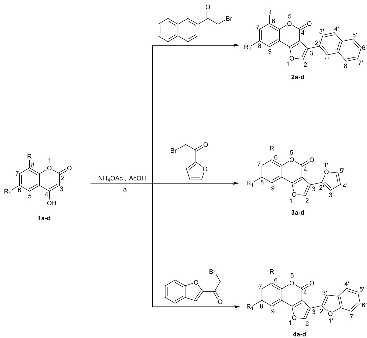
Scheme 1. 3-Aryl-furo[3,2-c]coumarins.
