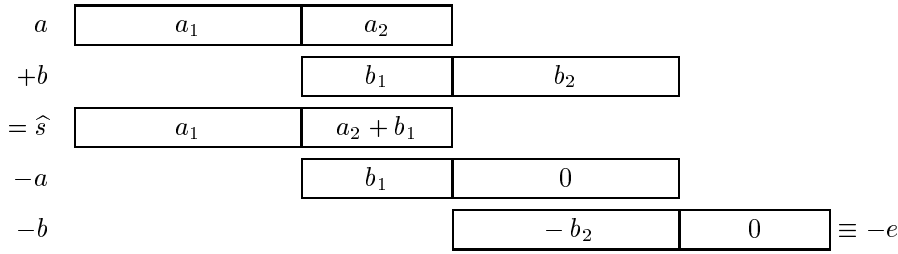
FIG. 3.1. Recovering the rounding error.
