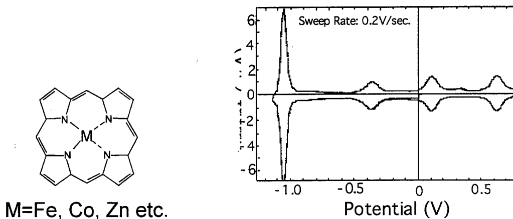
Figure 1. Left: Schematic of a transition metal porphyrin. Right: Electron transfer current between graphite electrode and tetrasulfonated iron phthalocyanine vs. the electrode potential in 0.05 M \text{KClO}_4 .
