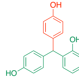
4,4'-((2-Hydroxyphenyl)methylene)diphenol (4bc) 1 H NMR (400 MHz, DMSO-d 6 )
