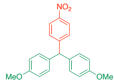
4,4'-((4-Nitrophenyl)methylene)bis(methoxybenzene) (3bi) 13 C NMR (100 MHz, DMSO-d 6 )
