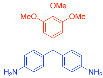
4,4'-((3,4,5-Trimethoxyphenyl)methylene)dianiline (3h) 1 H NMR (400 MHz, DMSO-d 6 )
