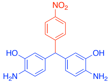
5,5'((4-Nitrophenyl)methylene)bis(2-aminophenol) (3q) 13 C NMR (100 MHz, DMSO-d 6 )
