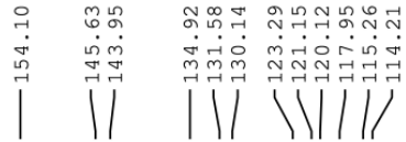
5,5'((4-Nitrophenyl)methylene)bis(2-aminophenol) (3q) 13 C NMR (100 MHz, DMSO-d 6 )
