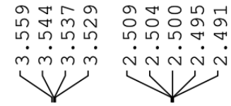
4,4'-((2-Hydroxyphenyl)methylene)diphenol (4bc) 1 H NMR (400 MHz, DMSO-d 6 )
