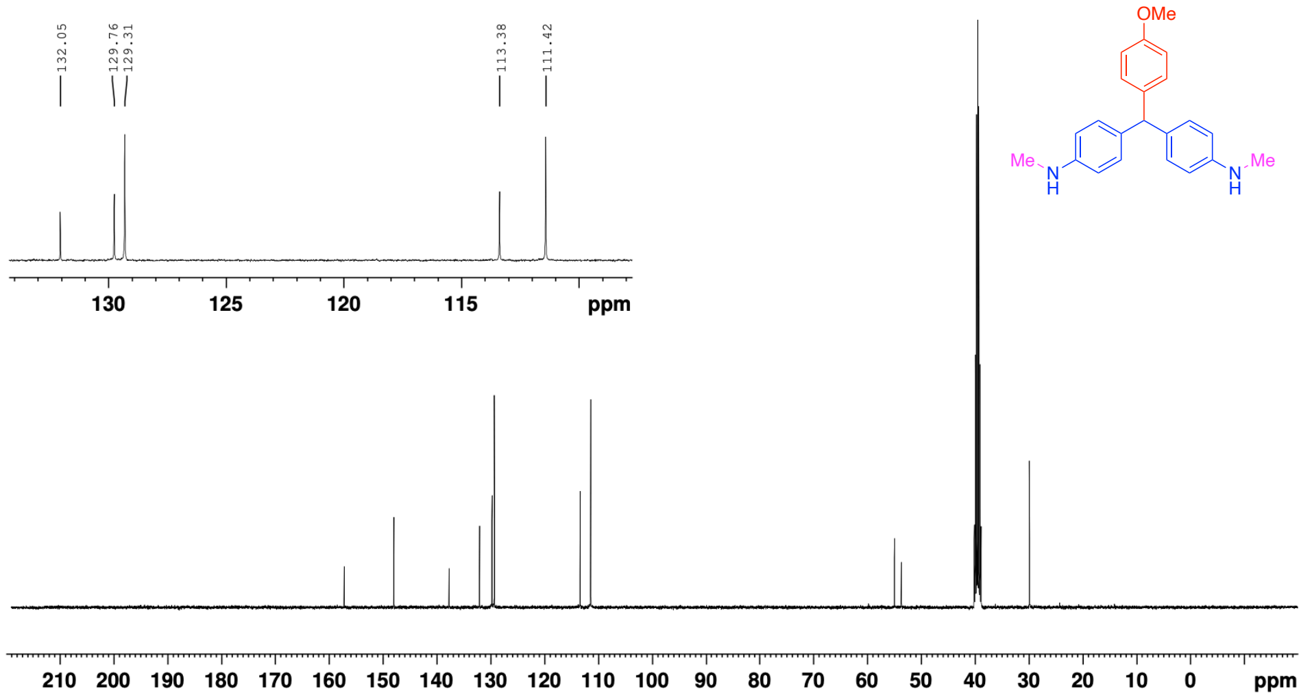
4,4'-((4-Methoxyphenyl)methylene)bis(N-methylaniline) (3ac) ^{13}\text{C} NMR (100 MHz, DMSO- d_6 )
