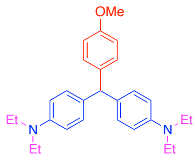
4,4-((4-methoxyphenyl)methylene)bis(N,N-diethylaniline) (3am) 13 C NMR (100 MHz, DMSO-d 6 )
