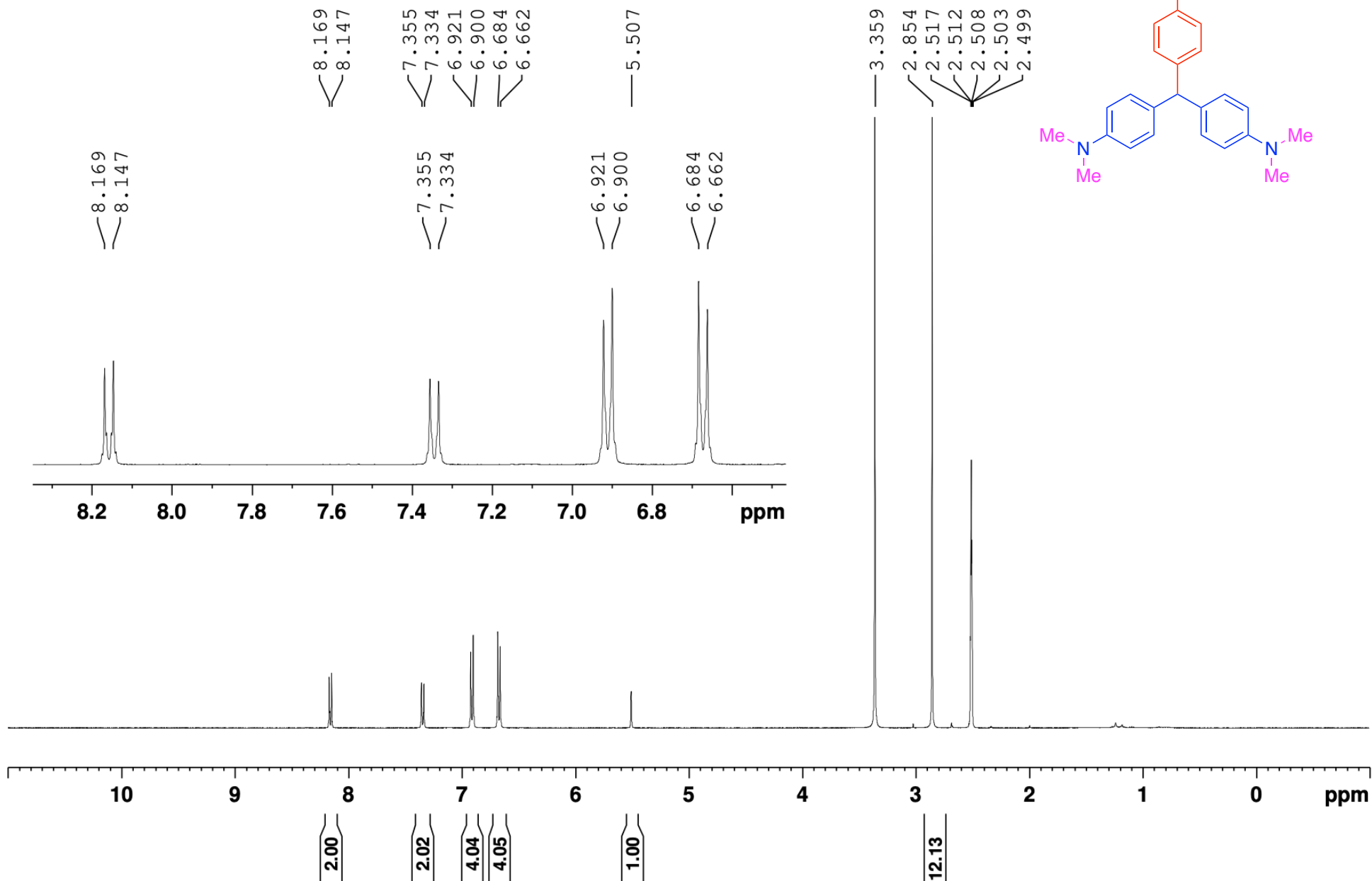
4,4'((4-Nitrophenyl)methylene)bis( N,N -dimethylaniline) (3ai) 1 H NMR (400 MHz, DMSO-d 6 )
