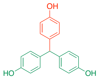
4,4',4''-Methanetriyltriphenol (3bc) 13 C NMR (100 MHz, DMSO-d 6 )
