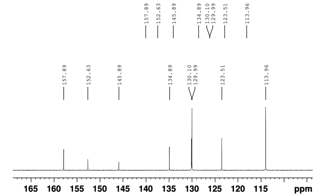
4,4'-((4-Nitrophenyl)methylene)bis(methoxybenzene) (3bi) 13 C NMR (100 MHz, DMSO-d 6 )
