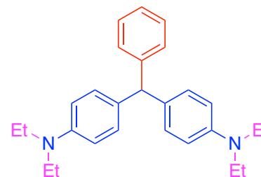
4,4'-(Phenylmethylene)bis( N,N -diethylaniline) (3ak) 13 C NMR (100 MHz, DMSO-d 6 )
