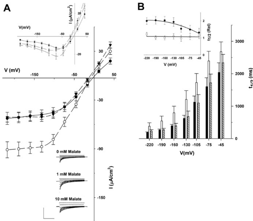
Figure 1 External Mal shows a biphasic modulation of I_{Cl} in Vicia guard cells
