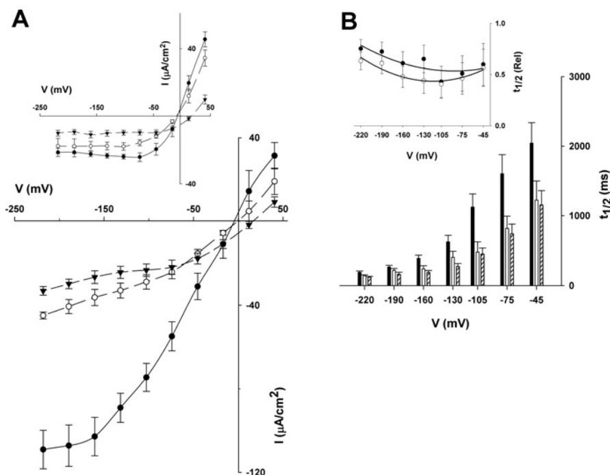
Figure 4 Internal OAA suppresses I_{\text{Cl}} at low millimolar concentrations in Vicia guard cells
