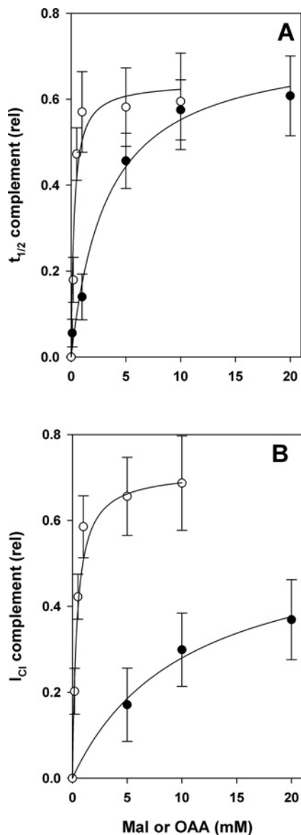
Figure 8 I_{Cl} in Vicia guard cells shows a high relative sensitivity to OAA (○) within the physiological concentration range compared with that for Mal (●)
