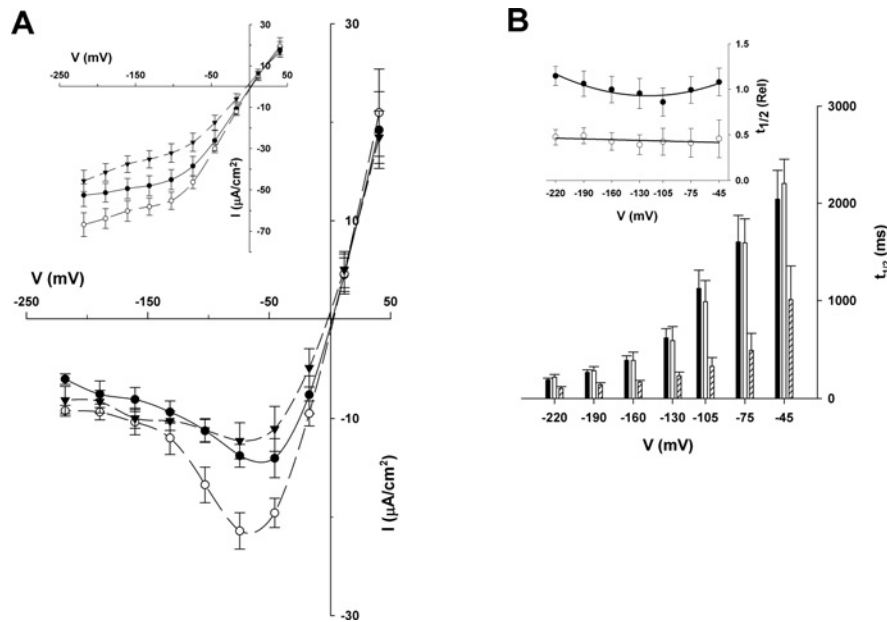
Figure 2 Internal Mal shows a marginal stimulation of I_{Ci} at low millimolar concentrations in Vicia guard cells
