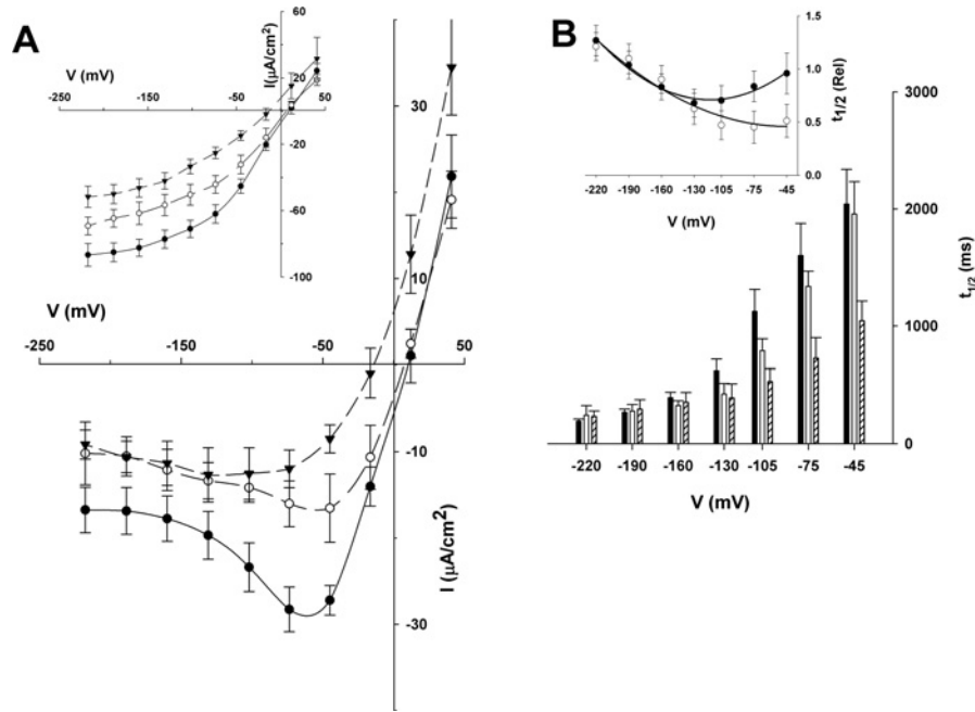
Figure 6 I_{Cl} in Vicia guard cells show a sensitivity to external Ac
