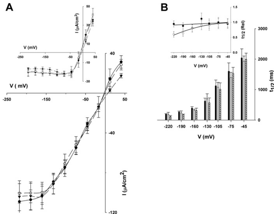
Figure 3 I_{Ci} in Vicia guard cells shows no appreciable sensitivity to external OAA
