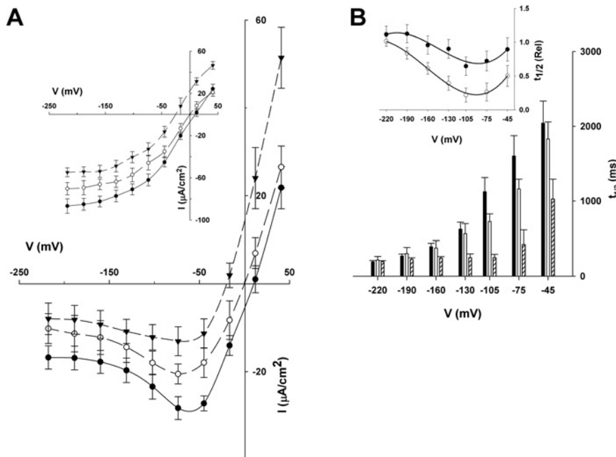
Figure 7 I_{Cl} in Vicia guard cells is suppressed by internal Ac
