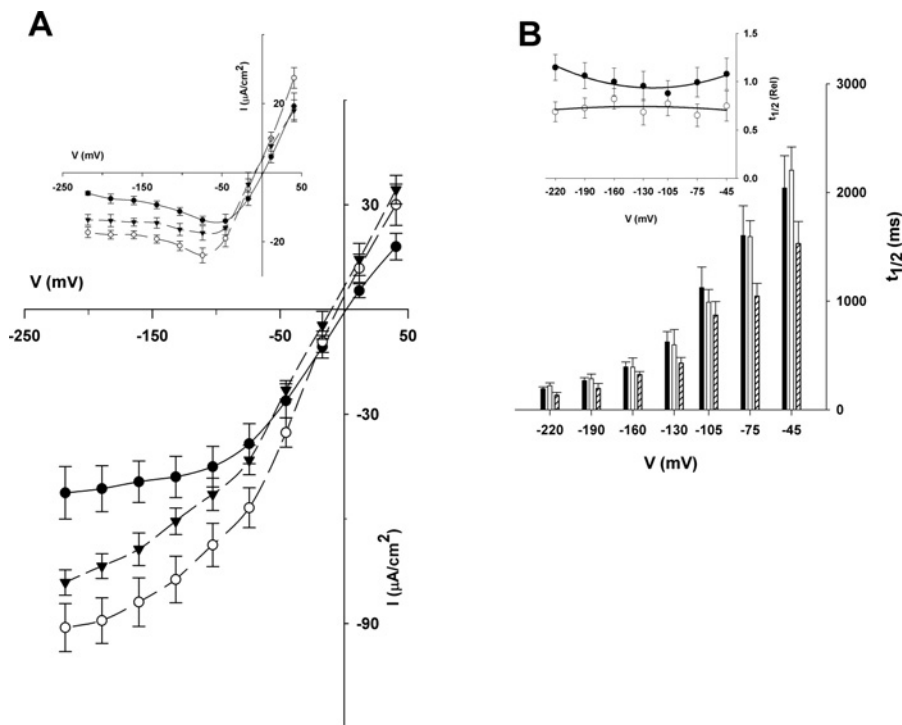
Figure 5 Internal OAA suppresses I_{Cl} in the presence of Mal in Vicia guard cells
