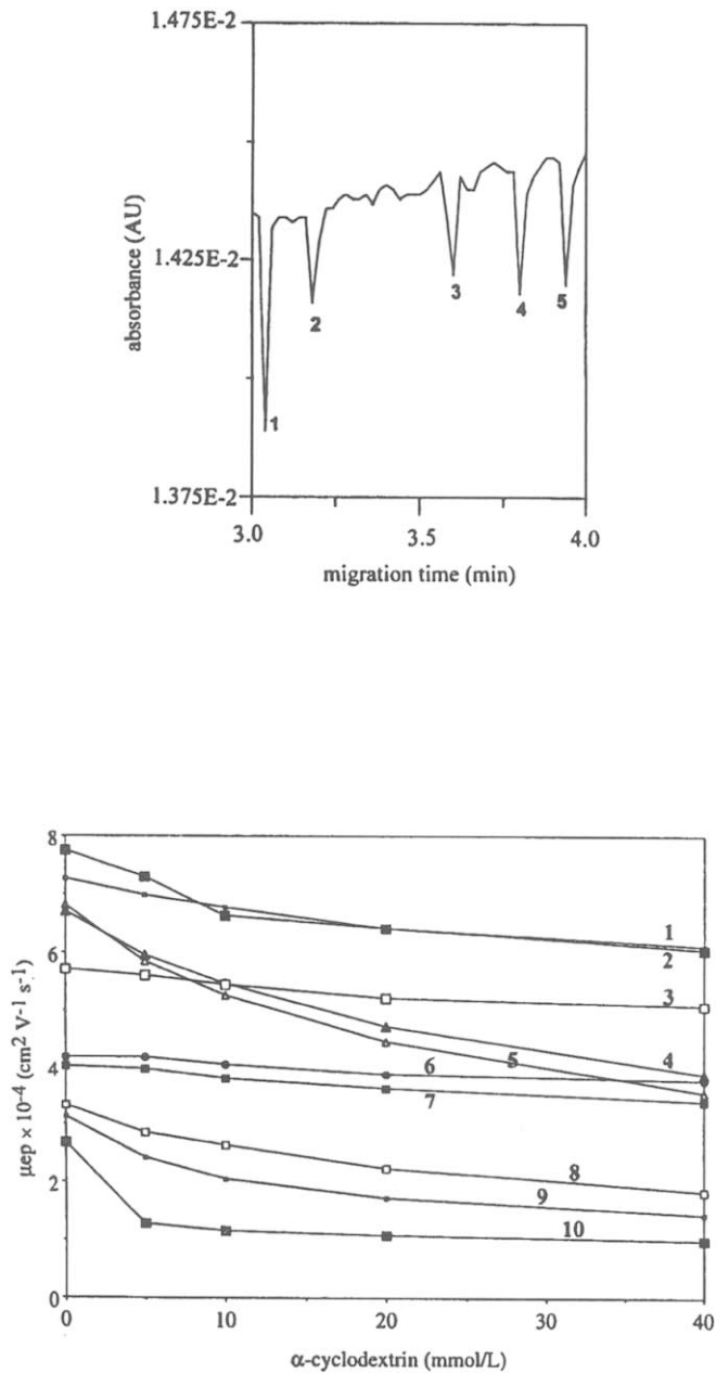
FIGURE 10. (A) Electropherogram of a mixture of anions (5 mM each) using \alpha -cyclodextrin to affect ionic mobility. Conditions: 5 mM sodium chromate, 20 mM \alpha -cyclodextrin, pH 8; hydrostatic injection for 15 s from a height of 10 cm ( \sim 100 \mu\text{M} ); applied electric field: 333 \text{ V cm}^{-1} . Peaks: 1 = nitrate, 2 = iodide, 3 = bromate, 4 = thiocyanate, 5 = perchlorate ( 500 \mu\text{g mL}^{-1} ). (B) Influence of \alpha -cyclodextrin concentration on electrophoretic mobility. Conditions: 5 mM potassium hydrogen phthalate + 0.002% poly(1,1-dimethyl-3,5-dimethylenepiperidinium chloride) (molar mass = 200 kDa), as electroosmotic flow modifier. Line identifications 1–5 see (A); 6 = iodate, 7 = ethanesulfonate, 8 = butanesulfonate, 9 = pentanesulfonate, 10 = octanesulfonate. (Reprinted from Can. J. Chem. 1998 , 76 , 194–198, with permission from the National Research Council of Canada © 1998.)
