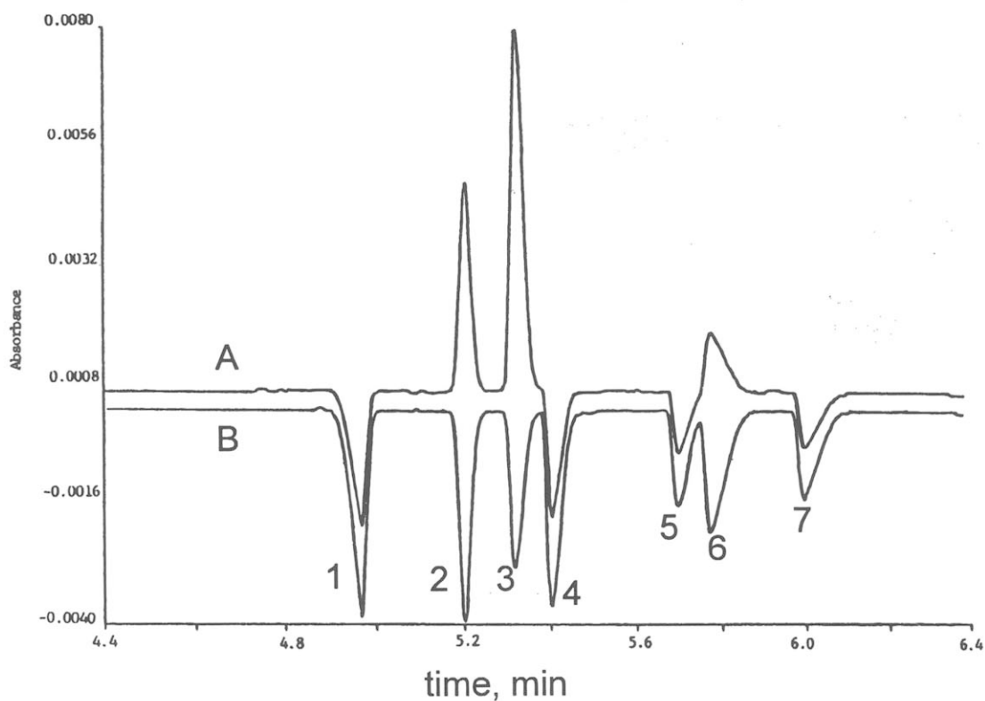
FIGURE 7. Electropherogram from the FBI Laboratory on a Dionex CES 1. Capillary: 65 cm \times 75 \mu m i.d.; Conditions: 3.6 mM chromate, 1 mM diethylenetriamine, borate buffer, pH 7.8; hydrostatic (gravity) injection: \sim 50 nL; indirect uv-detection: A = 205 nm; B = 280 nm. Peaks: 1 = chloride, 2 = nitrite, 3 = nitrate, 4 = sulfate, 5 = perchlorate , 6 = thiocyanate, 7 = chlorate. Note that nitrite, nitrate, and thiocyanate all absorb at 205 nm, thereby producing positive peaks. This additional information can be used to confirm or rule out identities obtained by elution time using the signal at 280 nm. Concentrations not reported. (Reprinted from J. Chromatogr. 1992 , 602 , 241–247, under U.S. government authority [not subject to copyright].)
