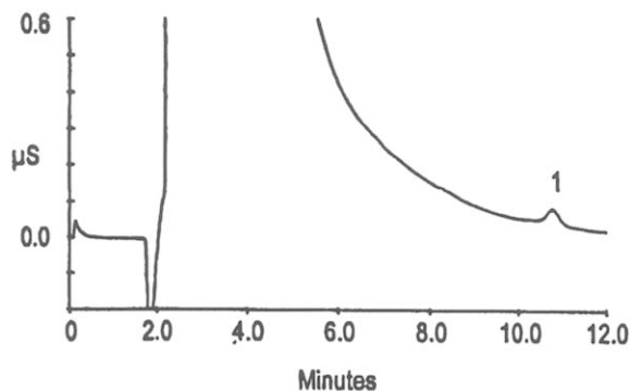
FIGURE 18. Ion chromatogram of 5 ng mL -1 perchlorate in synthetic ground water on the Dionex IonPac AG16 (guard) and AS16 (analytical) columns. Synthetic ground water contains 200 µg mL -1 chloride, 50 µg mL -1 nitrate, 200 µg mL -1 carbonate, 1000 µg mL -1 sulfate. Peak 1 = perchlorate. (Reprinted from J. Chromatogr. A 1999, 850, 131–135, with permission from Elsevier Science © 1999.)
