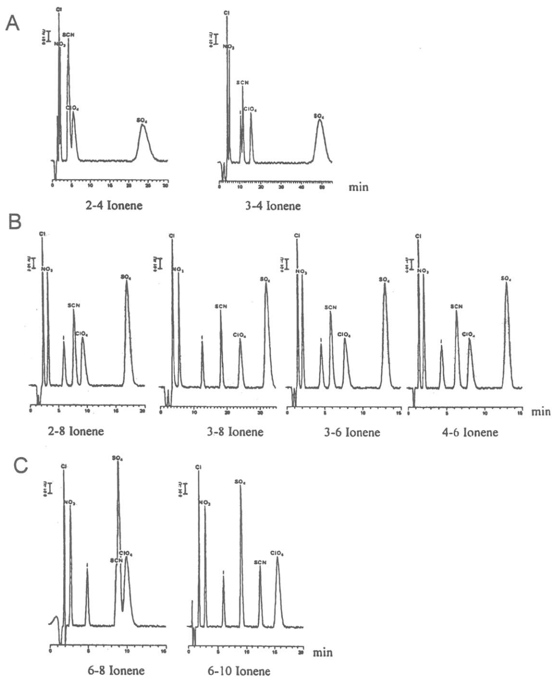
FIGURE 20. Typical ion chromatograms obtained using ionenes. Conditions: 3 \times 50 mm column packed with Silasorb S; 0.3 mM potassium hydrogen phthalate eluent; pH 6.8; flow rate 1.0 \text{ mL min}^{-1} ; uv-detection at 254 nm. (Reprinted from J. Chromatogr. A 1999 , 850, 53–63, with permission from Elsevier Science © 1999.)
