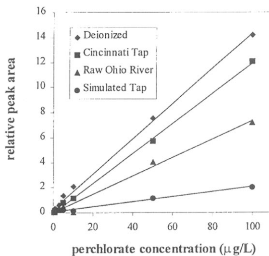
FIGURE 24. Single ion monitoring ( m/z = 380 u) by ESI-MS for the CH_2Cl_2 -extracted complex anion C_{10}H_{21}NMe_3(Br)(ClO_4)^- in several different water matrices. (Reprinted from Anal. Chem. 2000 , 72, 25–29, under U.S. government authority [not subject to copyright].)
