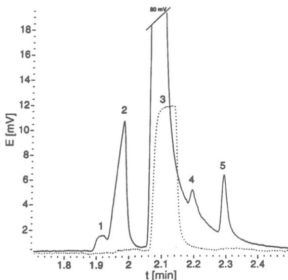
FIGURE 5. Electropherogram of 10 nM (1 ng mL -1 ) perchlorate in tap water (solid line). Detection by ion specific micro electrode. Conditions: running electrolyte: 20 mM sodium hydrogen sulfate/sodium sulfate, pH 2.5; electrokinetic injection potential: 10 kV for 10 s; separation potential: 30 kV; uncoated capillary. Dotted line shows effect of adding 20 mM sulfate. Peaks: 1 = bromide, 2 = chloride, 3 = nitrate, 4 = perchlorate , 5 = unknown. (Reprinted from J. Chromatogr. A 1994 , 676, 437-442, with permission from Elsevier Science © 1994.)
