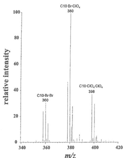
FIGURE 23. ESI mass spectrum of complex anions found when extracting perchlorate with decyltri methylammonium ion, C_{10}H_{21}N(CH_3)_3^+ , supplied as the bromide salt. Observable complexes contain two anions. Three different anionic complexes are seen: Br/Br, Br/ ClO_4 , and ClO_4/ClO_4 . (Reprinted from Anal. Chem. 2000 , 72, 25–29, under U.S. government authority [not subject to copyright].)
