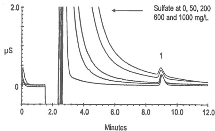
FIGURE 17. Ion chromatogram of 20 \text{ ng mL}^{-1} perchlorate on the Dionex IonPac AG11 (guard) and AS11 (analytical) columns. Conditions: 0.10 \text{ }\mu\text{M NaOH(aq)} eluent; flow rate: 1.0 \text{ mL min}^{-1} ; suppressed conductivity; 1000 \text{ }\mu\text{L} injection. Stacked chromatograms show the effect of adding sulfate (bottom to top) 0, 50, 200, 600, and 1000 \text{ }\mu\text{g mL}^{-1} . Peak 1 = perchlorate. (Reprinted from J. Chromatogr. A 1999 , 850 , 131–135, with permission from Elsevier Science © 1999.)
