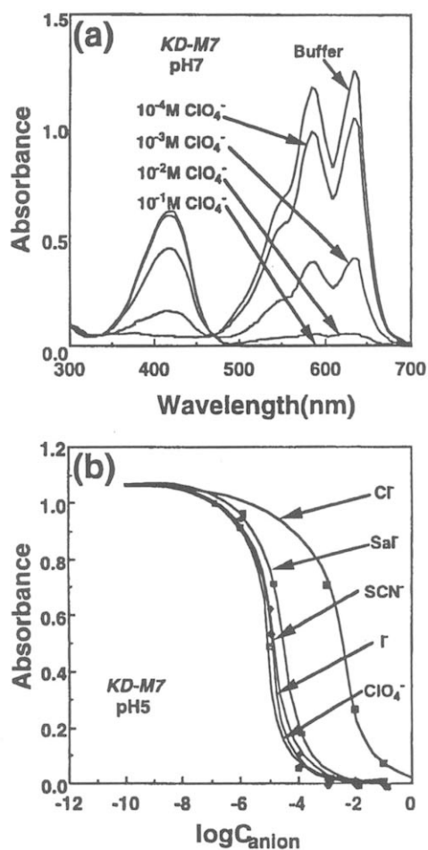
FIGURE 2. Typical characteristics of multi-information dyes used as optodes for perchlorate. \text{Sal}^- = salicylate. (Reprinted from Anal. Chim. Acta 1998 , 373, 271–289, with permission from Elsevier Science © 1998.)
