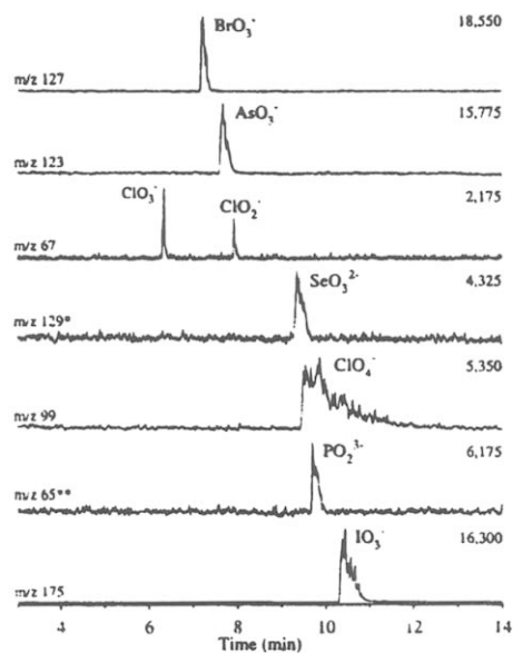
FIGURE 12. CE-ion spray-MS for inorganic anions (1 mM) using 2.5 mM pyromellitic acid in 20% MeOH, pH 7.8. *Singly protonated. **Doubly protonated. (Reprinted from Anal. Chem. 1996 , 68 , 2155–2163, with permission from the American Chemical Society © 1996.)
