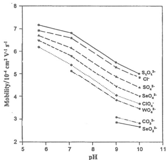
FIGURE 14. Electrophoretic mobility as a function of pH. Conditions: fused silica capillary covalently modified with [24]ane-N 6 × 50 cm (100 μm i.d.); 5 mM sodium chromate; applied potential: 15 kV; analyte concentration: 10 μM (1 μg mL -1 for perchlorate); electrokinetic injection for 5 s at -15 kV; indirect uv detection at 250 nm. (Reprinted from the Analyst 1997, 122, 1393–1398, with permission from the Royal Society of Chemistry © 1997.)
