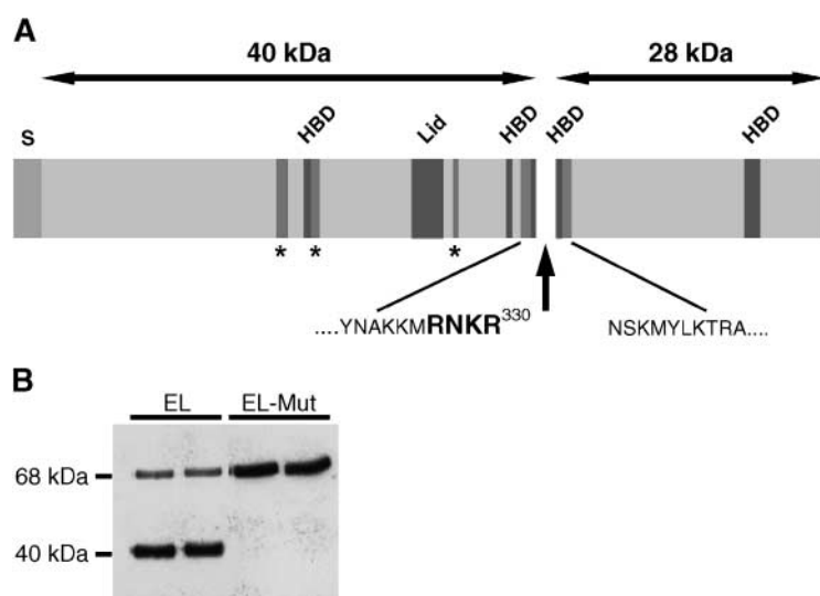
Fig. 3. Schematic presentation of the EL cleavage site together with the N- and C-terminal cleavage products (A) and effect of the Arg-330 \rightarrow Ser substitution on EL cleavage (B). A: The cleavage recognition sequence for proprotein convertases is indicated in boldface letters, and a vertical arrow indicates the cleavage site. Heparin binding domains are indicated by HBD, and the catalytic residues are indicated by asterisks. The numbering includes 20 amino acid residues of the signal peptide (S). Lid domain covers the catalytic site and confers substrate specificity to the enzyme. B: Heparin-supplemented medium of Hek-293 cells stably expressing EL- and EL-MUT-myc/His was concentrated in a SpeedVac and analyzed by Western blot as described for Fig. 1 using N-EL antibody and the ECL system.
