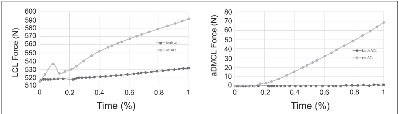
Figure 5 Simulation of the strain force for LCL (left) and aDMCL (right) during the Lachman test which are the main restrictors in the absence of ACL bundles
