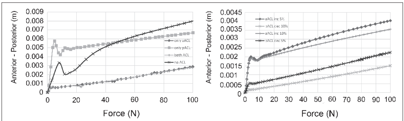
Figure 4 The diagrams show the anterior-posterior displacement with respect to the force applied to the posterior aspect of the proximal tibia during the Lachman test simulation for different surgical choices. On the left diagram the response of the model is investigated based on the insertion of single or double bundles for the ACL ligament. On the right diagram an investigation is made by adjusting the restraining length of the two bundles, by increasing or decreasing the initial resting length.
