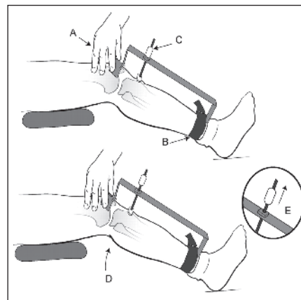
Figure 2 Rolimeter configuration during Lachman test
