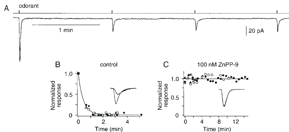
Figure 5 LLA of the odor response of an intact ORN. (A) Response of an individual ORN to four repeated 100 ms odor pulses (cineole, 100 \mu M) plotted at low time resolution. Note that, despite the fact that the interpulse interval was >1 min, which is sufficient to allow for recovery from early forms of adaptation, the response to the second stimulus nonetheless was strongly reduced compared with the response to the first pulse. There was no further decrement in the responses to subsequent stimuli. This adaptive effect was fully reversible after 6 min in odor-free solution (not shown). (B) Plot of the onset time course of LLA under control conditions. Data are from six cells (shown with different symbols). Cells are stimulated with 300 \mu M cineole. Odor responses of a given cell are normalized to (I - I_{LLA}) / (I_{control} - I_{LLA}) , so that the incremental peak response under control conditions ( I_{control} ) is set to the value one and the mean equilibrium peak response after producing LLA ( I_{LLA} ) is given the value zero. The continuous line is a best fit of the data with a single exponential function giving a time constant \tau = 24 s. Insets are representative waveforms of transient odor-induced currents taken before LLA (large response) and after LLA was established (small response). (C) Effect of ZnPP-9 (100 nM, n = 4 ) on LLA demonstrating that LLA is abolished after ZnPP-9 treatment in all tested cells. The solid line was computed by regression analysis. Insets demonstrate that the characteristic properties of the cAMP-mediated response remain unchanged during ZnPP-9 treatment and that there is no response decrement over time (the second response was taken 12 min after the first). Modified from (Zufall and Leinders-Zufall, 1997).
