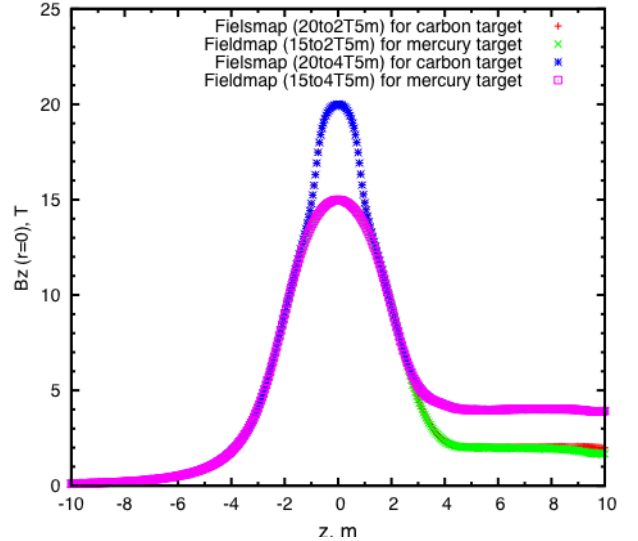
Figure 2: Axial magnetic field of the 20to2T5m and 20to4T5m configurations for a C target, and of the 15to2T5m and 15to4T5m configurations for an Hg target.. The center of the target is at z = 0 .
