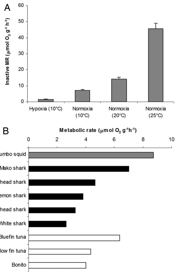
Fig. 2. Inactive mass-specific oxygen consumption rates (IMR, \mu\text{mol O}_2 \text{g}^{-1} \text{h}^{-1} ) in jumbo squid, Dosidicus gigas . (A) Effect of temperature and oxygen (hypoxia, 1% \text{O}_2 ; normoxia, 21% \text{O}_2 ) on IMR. Values are means \pm SE (more details in supporting online material, Table S2). (B) Comparison of estimated IMR ( \mu\text{mol O}_2 \text{g}^{-1} \text{h}^{-1} ) of jumbo squid and the standard metabolic rate (calculated by extrapolating to zero speed) of other top predators in the Eastern Tropical Pacific (ETP) (sources for shark and tuna data are available in Table S3). Rates were estimated for 1-kg animals and standardized to 20°C, assuming a Q_{10} of 2 and a scaling coefficient of -0.25 for fishes. For D. gigas , the extrapolation to bigger size was based on the common tendency for isometric metabolic scaling ( \text{IMR} = aM^{0.04} at 20°C, Table S2) in muscular squids (22).
