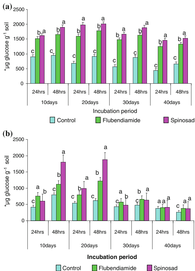
Fig. 2 Influence of flubendiamide and spinosad on invertase*activity in a black clay and b red clay soil at 2.5 \text{ kg ha}^{-1} . * \mu\text{g} glucose per gram soil formed after 24 and 48 h incubation with 18 Mm sucrose. The values are the mean \pm SE for each incubation period, are not significantly different ( P \leq 0.05 ) from each other according to Duncan's multiple range (DMR) test
