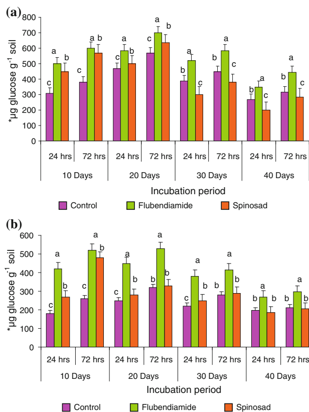
Fig. 3 Influence of flubendiamide and spinosad on amylase activity in a black clay and b red clay soil at 2.5 kg ha -1 . *µg glucose per gram soil formed after 24 and 72 h incubation with 2 % starch. The values are the mean ± SE for each incubation period, are not significantly different ( P \leq 0.05 ) from each other according to Duncan's multiple range (DMR) test
