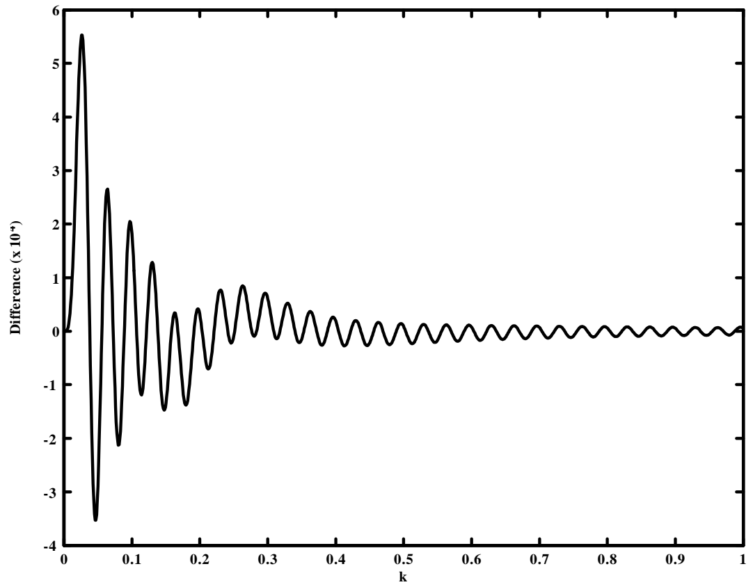
Figure 2: Difference between the analytical and approximate 4th order Hankel transform of the selected Laguerre function.
