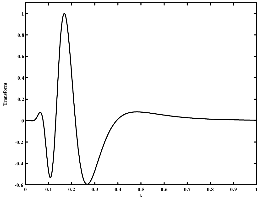
Figure 1: Approximate 4th order Hankel transform of a Laguerre function obtained from the Zernike expansion.
