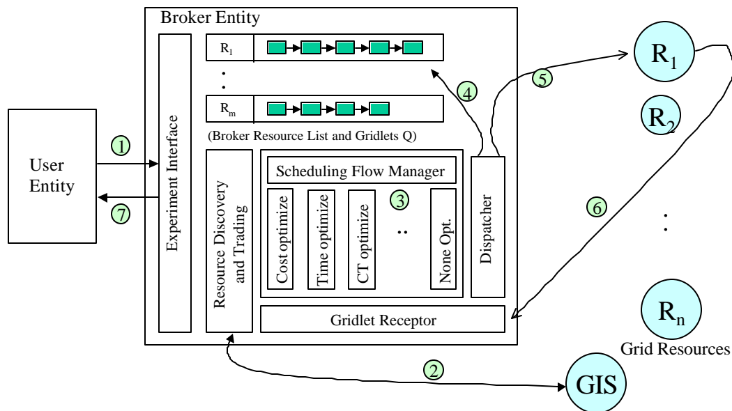
Figure 18: Economic grid resource broker architecture and its interaction with other entities.
