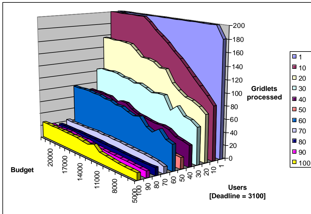
Figure 33: No. of Gridlets processed for each user when a varying number of users competing for resources.
