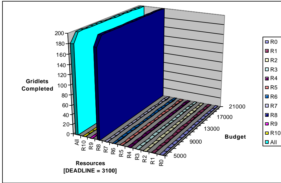
Figure 27: Gridlets processed on resources for different budget values with high deadline.
