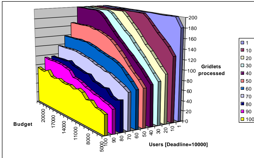
Figure 36: No. of Gridlets processed for each user with varying number of users competing for resources.
