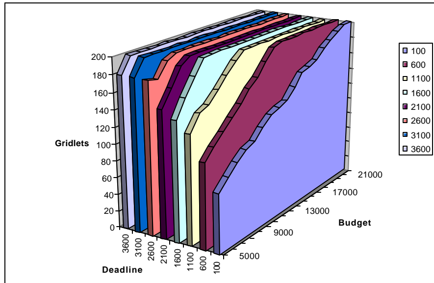
Figure 21: No. of Gridlets processed for different budget limits with a fixed deadline for each.
