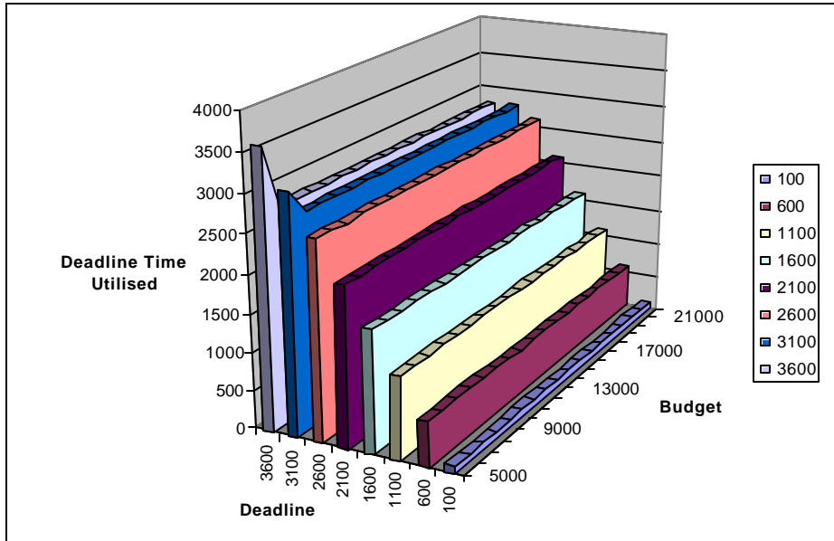
Figure 23: Deadline time utilized for processing Gridlets for different values of deadline and budget.
