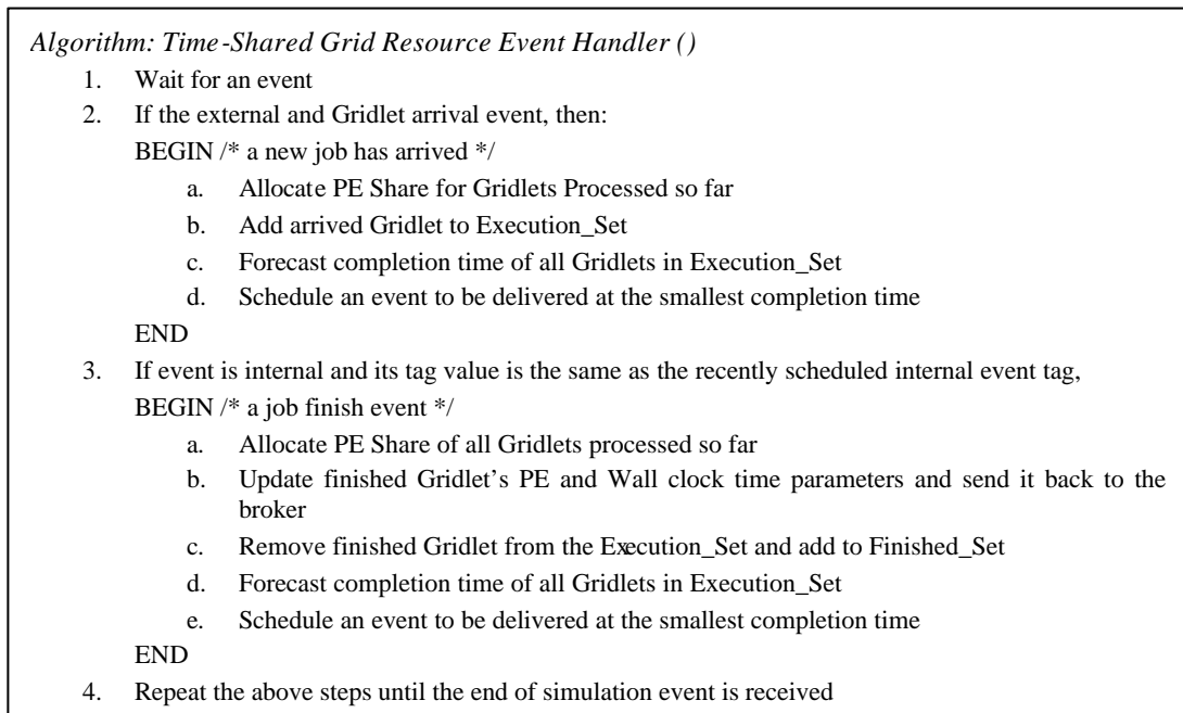
Figure 7: An event handler for simulating time-shared resource scheduling.
