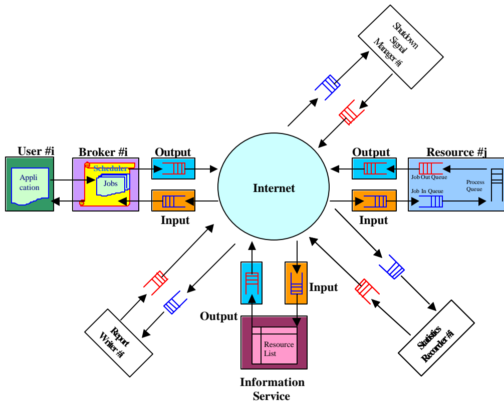
Figure 3: A flow diagram in GridSim based simulations.
