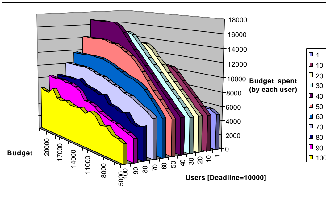
Figure 38: The average budget spent by each user for processing Gridlets.
