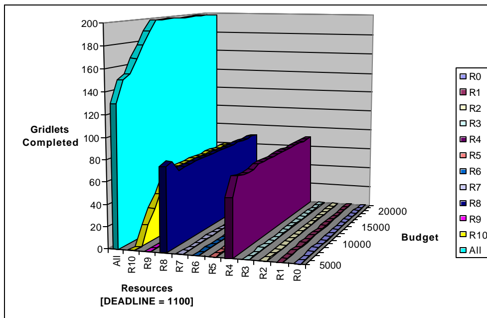
Figure 26: Gridlets processed on resources for different budget values with medium deadline.
