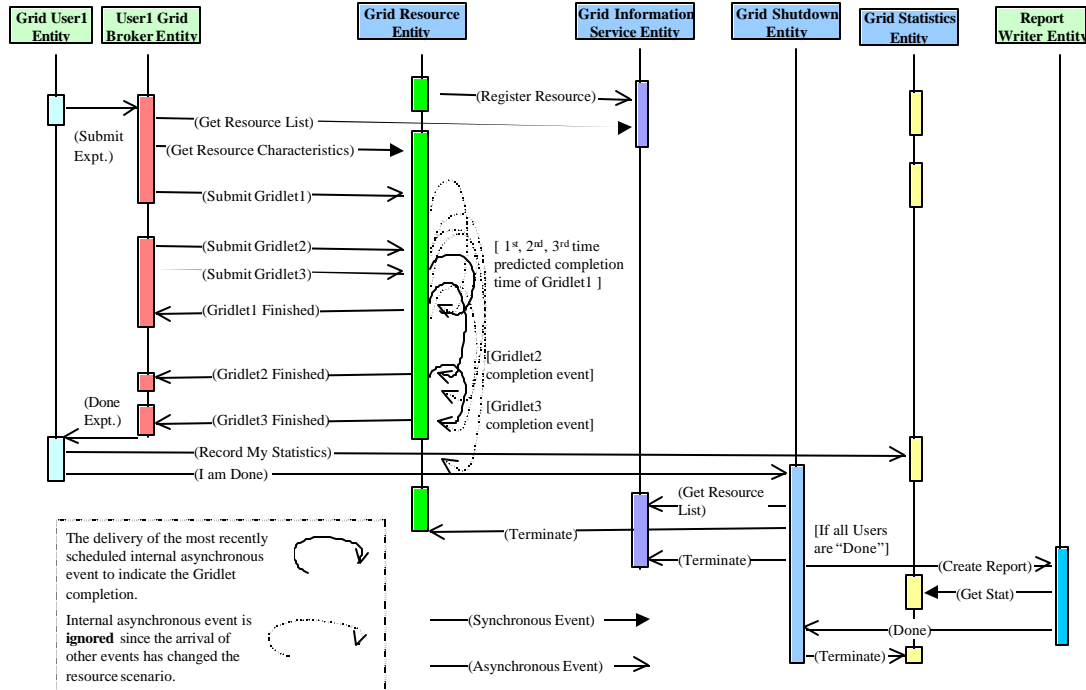
Figure 5: An event diagram for interaction between a time-shared resource and other entities.
