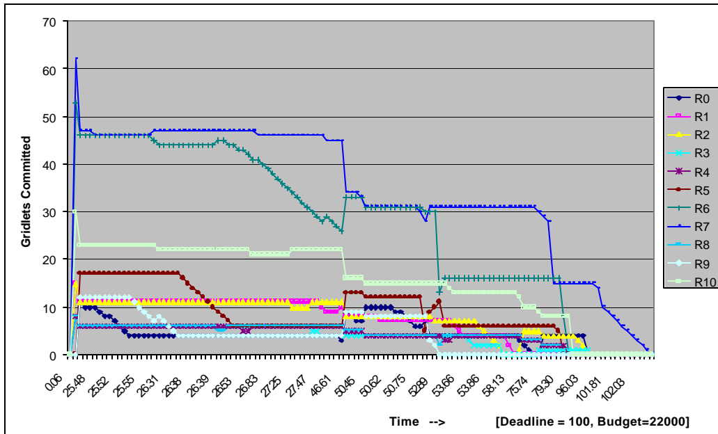
Figure 31: Trace of the number of Gridlets committed to resources for a low deadline and high budget constraints.
