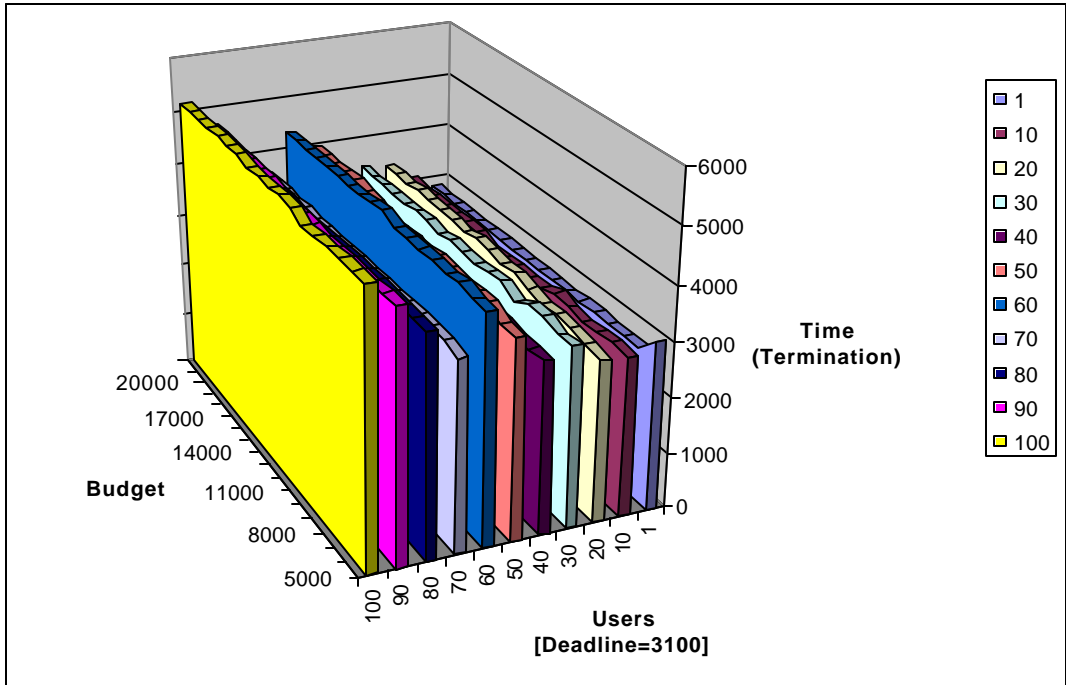
Figure 34: The average time at which the user experiment is terminated with varying number of users competing for resources. When there are a large number of users arriving at different times, they are likely to impact on the schedule and the execution time of jobs already deployed on resources. The broker waiting for the return of jobs that are deployed on resources leads to the termination time exceeding the soft deadline unless the execution of jobs is cancelled immediately.
