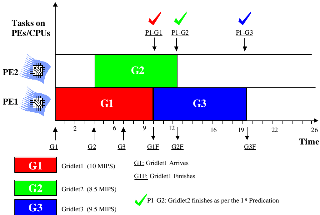
Figure 12: Modeling space-shared multiprocessing based on an event scheme.
