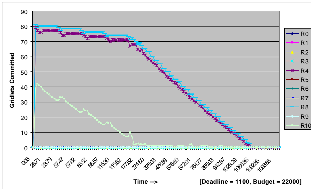
Figure 32: Trace of the number of Gridlets committed to resources for a medium deadline and high budget constraints.
