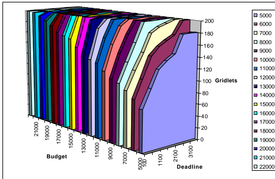
Figure 22: No. of Gridlets processed for different deadline limits with a fixed budget for each.
