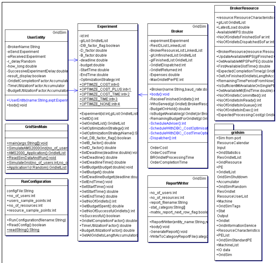
Figure 19: A class hierarchy diagram of Grid broker using the gridsim package.
