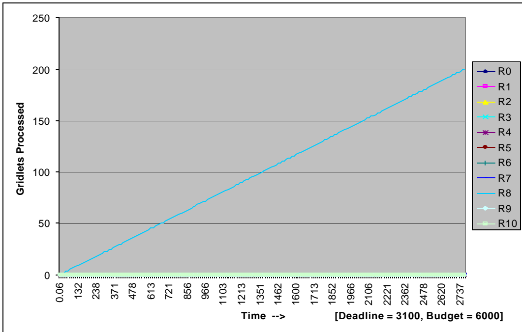
Figure 30: Trace of No. of Gridlets processed for a high deadline and low budget constraints.
