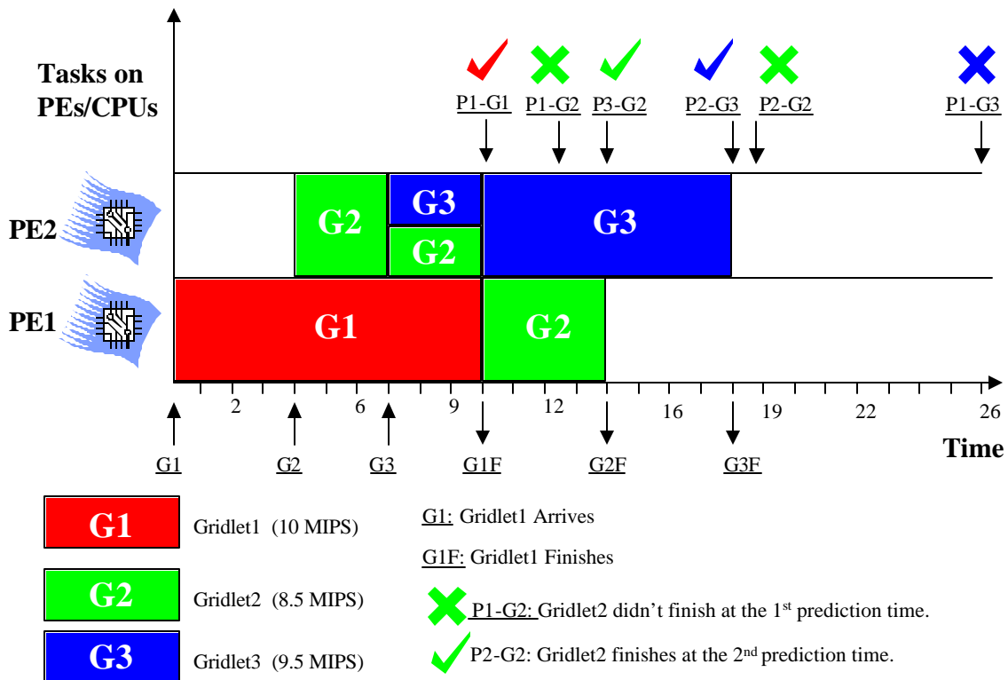
Figure 9: Modeling time-shared multitasking and multiprocessing based on an event scheme.
