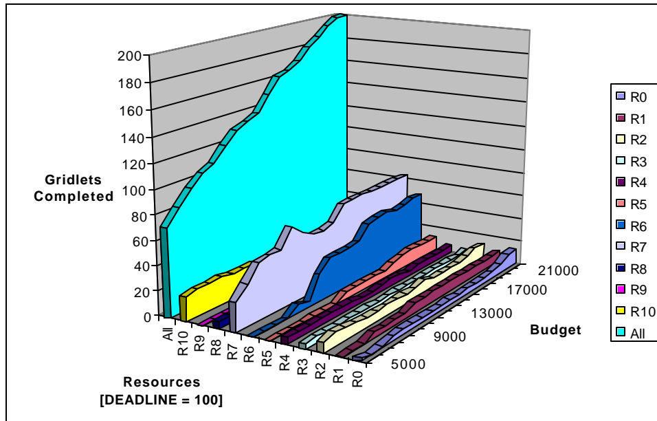
Figure 25: Gridlets processed on resources for different budget values with low deadline.
