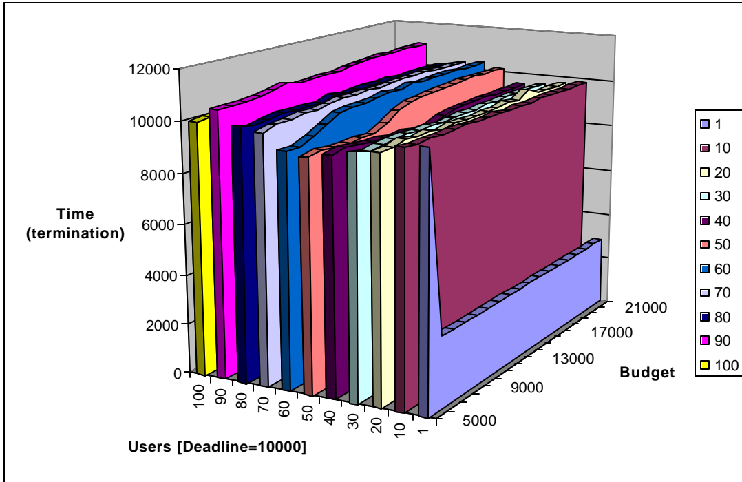
Figure 37: The average time at which the user experiment is terminated with varying number of users competing for resources.
