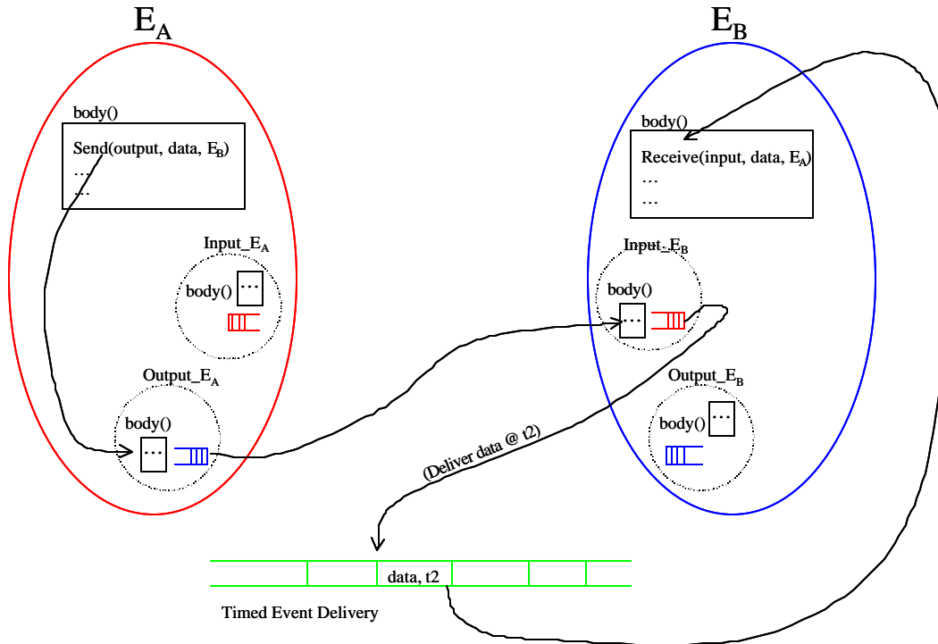
Figure 4: Entity communication model via its Input and Output entities.
