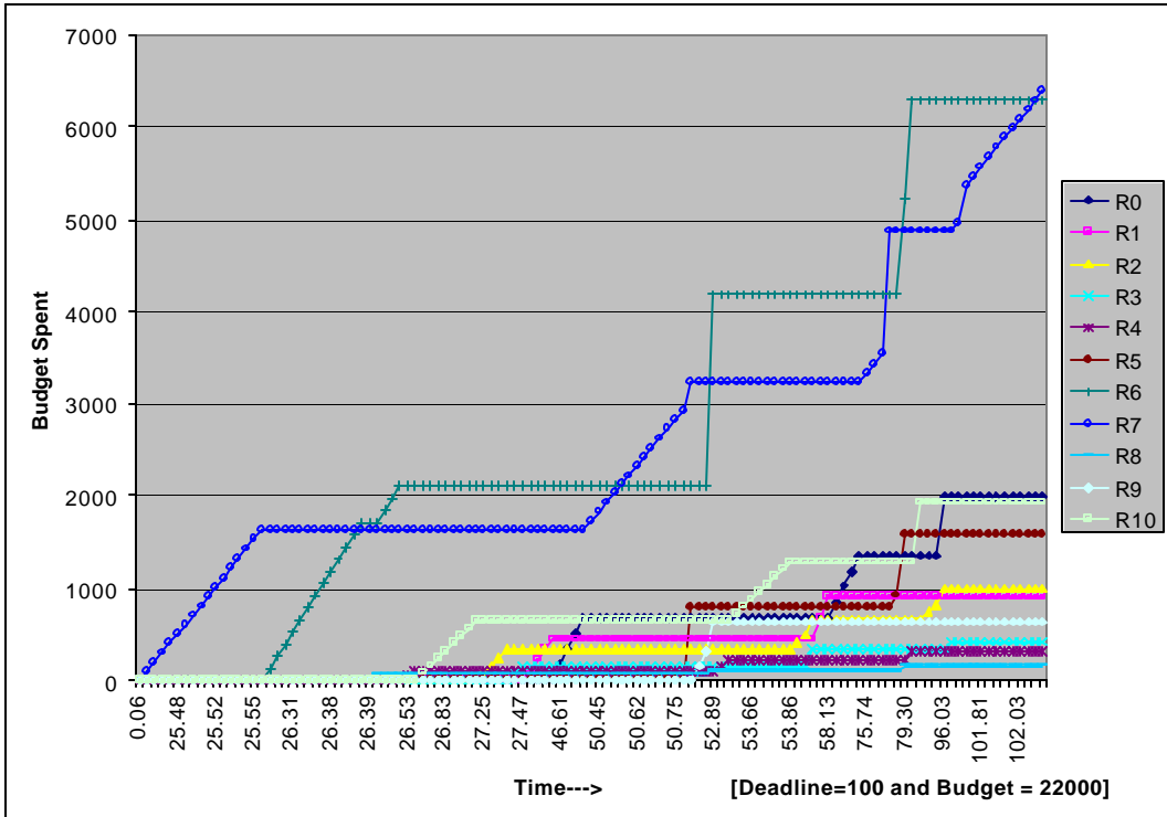
Figure 29: Trace of budget spent for low deadline and high budget constraints.
