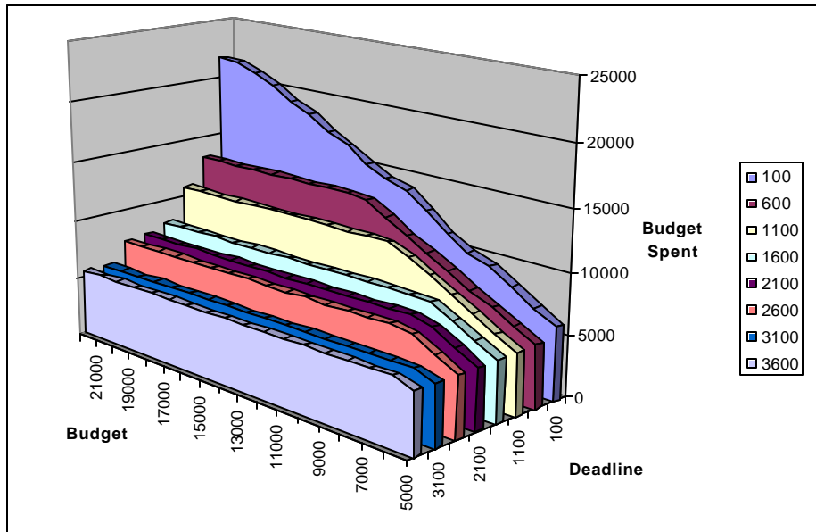
Figure 24: Budget spent for processing Gridlets for different values of deadline and budget.
