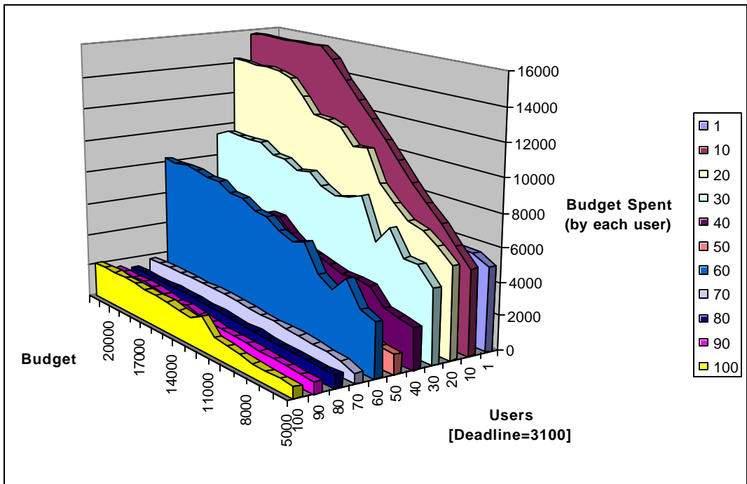
Figure 35: The average budget spent by each user for processing Gridlets.
