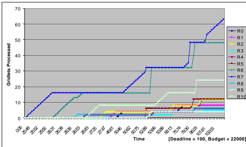
Figure 28: Trace of No. of Gridlets processed on resources for a low deadline and high budget constraints.
