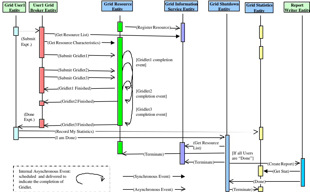
Figure 6: An event diagram for interaction between a space-shared resource and other entities.
