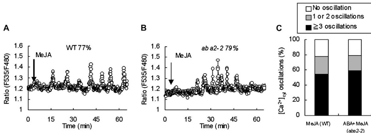
Figure 6. Effect of 0.1 µM ABA on MeJA-induced [Ca^{2+}]_{cyt} oscillations in aba2-2 guard cells. A, Representative data of fluorescence emission ratio (535/480 nm) showing [Ca^{2+}]_{cyt} oscillations in 10 µM MeJA-treated wild-type (WT) guard cells ( n = 17 of 22 cells; 77%). B, Representative data of fluorescence emission ratio (535/480 nm) showing MeJA-elicited [Ca^{2+}]_{cyt} oscillations in aba2-2 guard cells treated with 0.1 µM ABA ( n = 19 of 24 cells; 79%). C, Stack column representation of MeJA-induced [Ca^{2+}]_{cyt} oscillations (%) in wild-type and aba2-2 guard cells in the absence (WT; n = 22 ) or presence ( aba2-2 ; n = 24 ) of 0.1 µM ABA.
