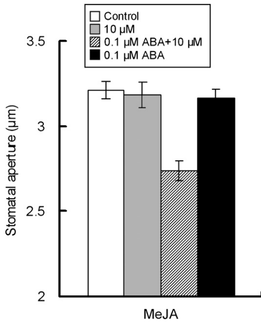
Figure 5. Effect of 0.1 µM ABA on MeJA-induced stomatal closure in aba2-2 guard cells. Rosette leaves of aba2-2 plants were treated with 0.1 µM ABA for 30 min. Then, rosette leaves pretreated with 0.1 µM ABA were incubated with 10 µM MeJA. Twenty averages from three independent experiments (60 total stomata per bar) are shown. Error bars represent SE.
