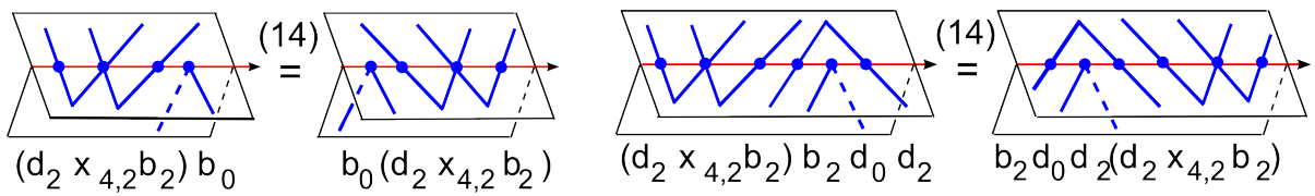
Figure 26: Relations (14) in the semigroup of Theorem 14.
