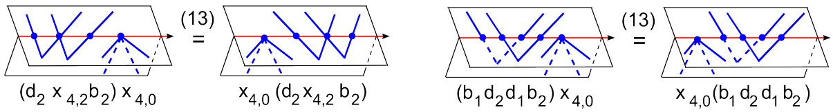
Figure 25: Relations (13) in the semigroup of Theorem 14.
