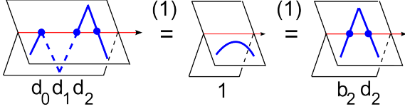
Figure 15: Relations (1) in the semigroup of Theorem 14.
