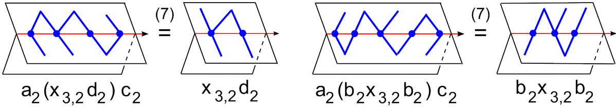
Figure 20: Relations (7) in the semigroup of Theorem 14.
