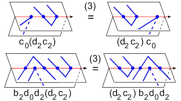
Figure 17: Relations (3) in the semigroup of Theorem 14.
