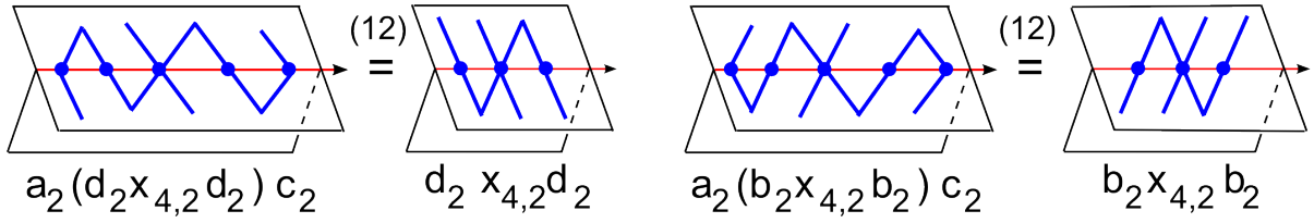
Figure 24: Relations (12) in the semigroup of Theorem 14.
