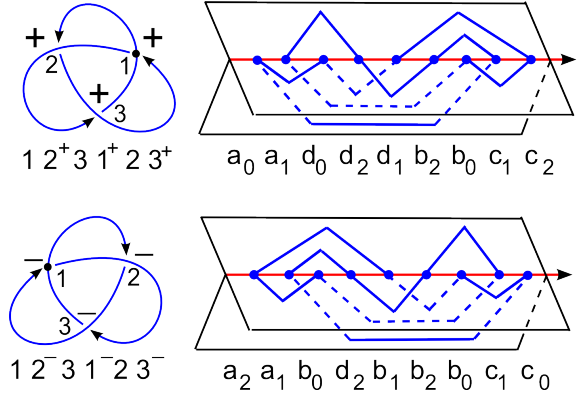
Figure 13: Trefoils, Gauss codes, 3-page embeddings
