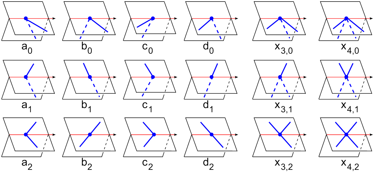
Figure 11: Local 3-page embeddings for the generators of the semigroups from Theorem 14.
