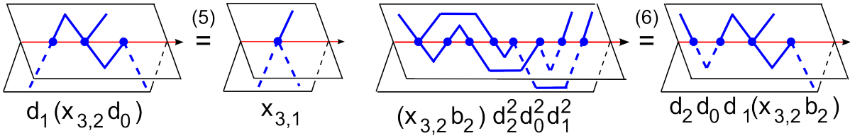
Figure 19: Relations (5)-(6) in the semigroup of Theorem 14.
