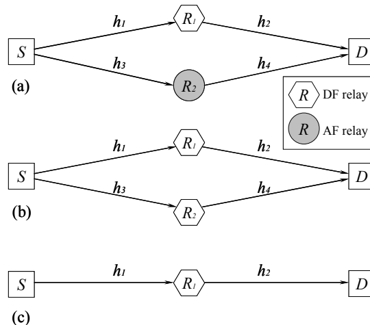
Fig. 8. hybrid DF-AF cooperation and DF cooperation architectures with different average power gains. (a) hybrid DF-AF cooperation, (b) dual DF cooperation, (c) single DF cooperation. (S: Source, D: Destination, h : average power gain between two nodes).
