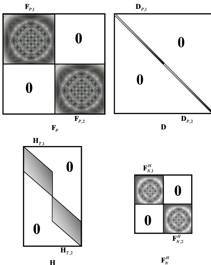
Fig. 14. Structures of the FFT matrices, CFOs matrix and channel matrix for 2-relay cooperative system, top left: FFT matrix F_P , top right: CFOs matrix D , bottom left: channel matrix: H , bottom right: FFT matrix F_N^H . Blank parts are all 0's.
